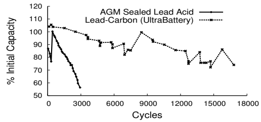
Figure 14: Comparison of sealed lead-acid and lead-carbon battery lifetime. Data from [21].
