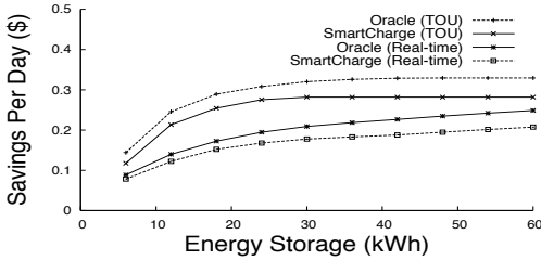
Figure 6: Average dollar savings per day for both real-time and TOU prices in our case study home.
