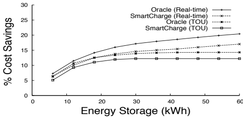
Figure 7: Average percentage savings for both real-time and TOU prices in our case study home.
