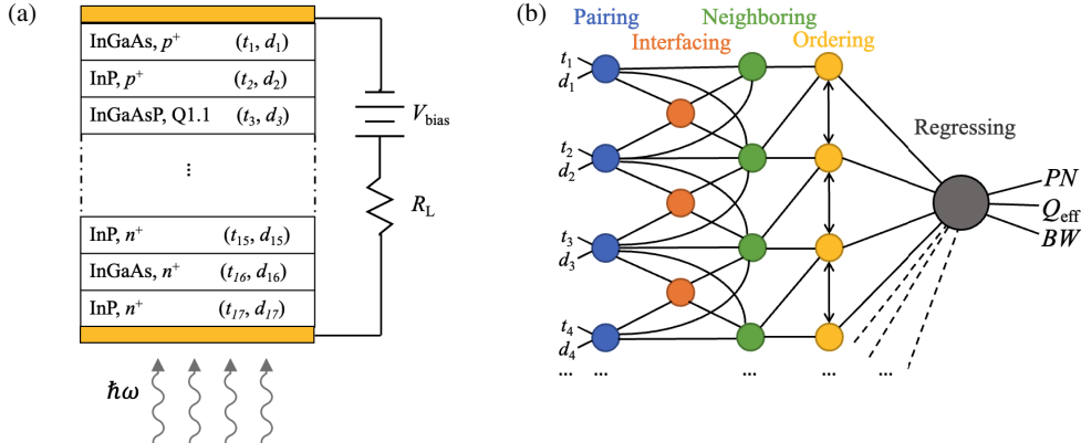
Figure 1: (a) A schematic of the MUTC photodetector with varying layer thicknesses and doping concentrations, t_i and d_i , respectively, for i = 1, 2, 3, \dots, 17 , and (b) an illustration of the neural network specifically designed to learn from device parameters to predict performance metrics such as the phase noise ( PN ), quantum efficiency ( Q_{eff} ), bandwidth ( BW ), etc.
