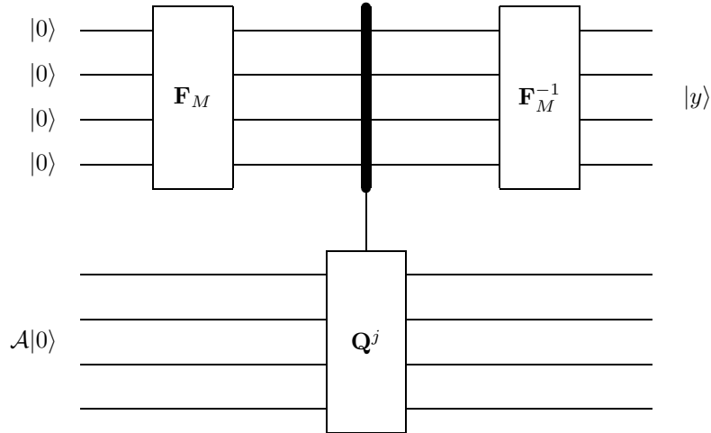
FIGURE 1. Quantum circuit for amplitude estimation.
