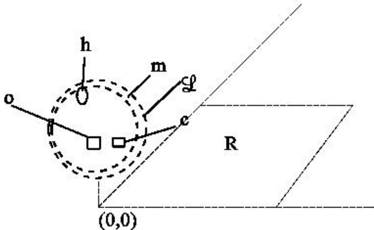
FIGURE 1. A Schematic Model of a Quantum Robot at the Origin of R . Both the memory system lattice ( m ) and Quantum Turing machine lattice \mathcal{L} are shown with the head h that moves on the lattices. The control qubit ( c ) and output system ( o ) are also shown. The quantum robot is greatly magnified relative to R to show details.
