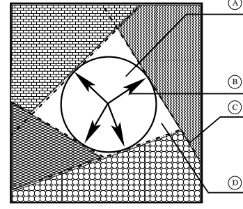
Figure 1: (A) the area inside an \epsilon circle (B) A random vector (C) A tangent defining a half-space (D) The areas between the circle and the union of half-spaces are the tie areas.
