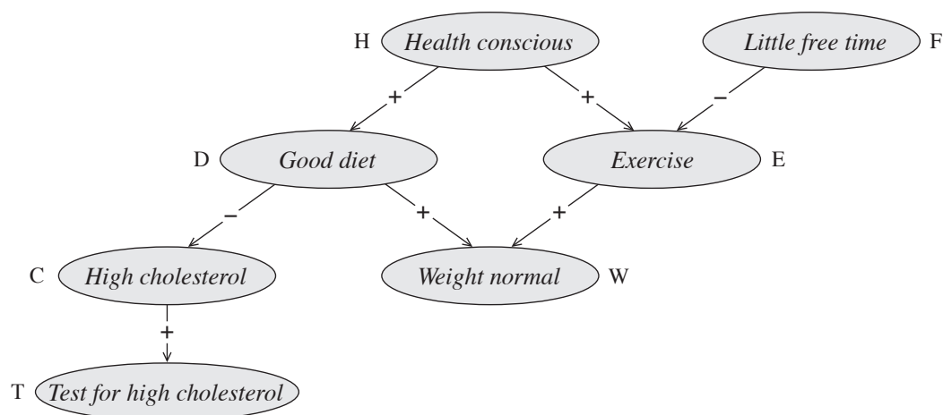
Figure 3.14 A Bayesian network with qualitative influences
