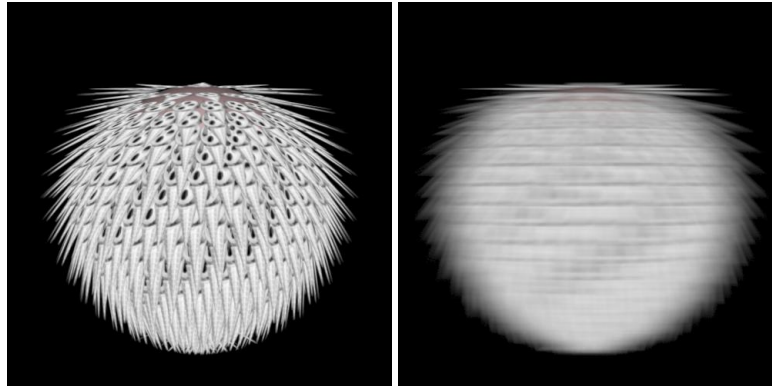
Figure 7.12: A case where our algorithm performs poorly: many stacked motion-blurred transparent objects. The “feathers” are rectangular strips that use a texture to modulate transparency.
