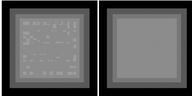
Figure 7.5: Exaggerated artifacts of opacity thresholding by batches. A stack of camera-facing planes, each with opacity 0.1, with the opacity threshold is set to the unreasonably low value of 0.2. Image on right shows the ideal solution.
