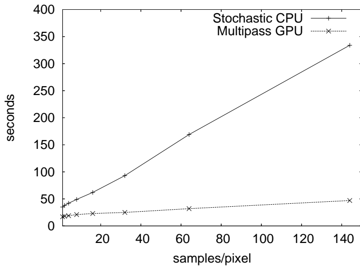
Figure 7.9: Performance comparison of our GPU-assisted multipass algorithm versus a CPU-only stochastic point sampling renderer (PRMan), rendering the displayed frame at 1800 \times 1080 pixels with 1, 2, 4, 8, 16, 32, 64, and 144 samples per pixel. Total render time minus shading delta.
