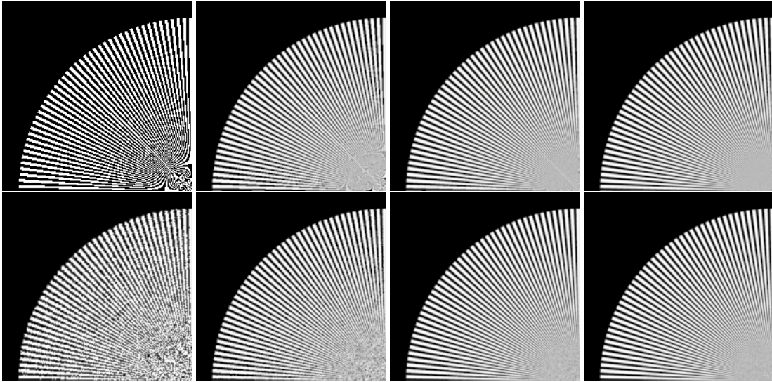
Figure 7.7: Antialiasing quality with 1, 4, 16, and 32 samples per pixel. Top: regular sampling; bottom: stochastic sampling.
