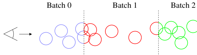
Figure 7.3: Clipping planes in z let us depth-peel each z -batch independently. Here we see three z -batches, with B = 5 . Assume each sphere is one grid. Note that grids that “trail” into a following batch are rendered in both batches, with z -clipping at the batch boundary.
