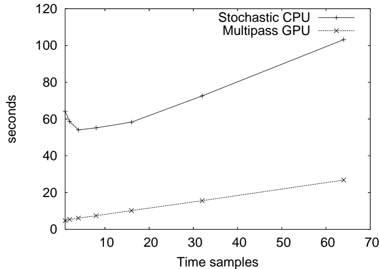
Figure 7.10: Motion blur performance, rendering the full creature shown cropped in Figure 7.8 at 1024 \times 786 pixels. The CPU renderer uses the same samples for time and space; the GPU renderer was run with 16 pixels per sample.
