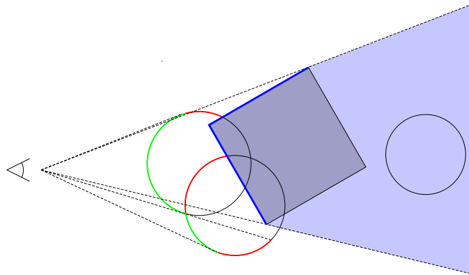
Figure 7.2: Depth peeling of three transparent spheres and an opaque cube, after one layer has been peeled. Green indicates the layers-so-far buffer (nearest layer) while red indicates the layer being computed (second-nearest layer). The blue line on the surface of the cube indicates the opaque-surfaces buffer, which culls away all surfaces behind it.
