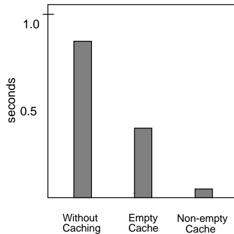
Figure 5: Cache performance is measured for three cases: (a) the without caching or base-line case where caching was disabled, (b) the empty cache case where caching was enabled but the cache was cleared before each repetition of the test set, and (c) the non-empty cache case where the cache contained the results for all queries in the test set.
