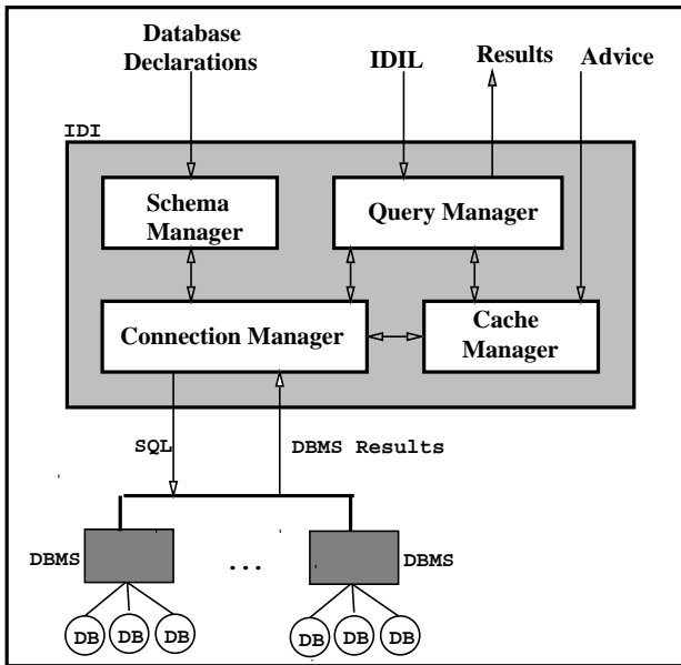
Figure 3: The IDI includes four main components: the Schema Manager manages the schema information for all declared databases; the Connection Manager handles connections to remote DBMSs; the Query Manager is responsible for processing IDIL queries and their results; and the Cache Manager controls the cache of query results in accordance with the advice supplied by the application.
