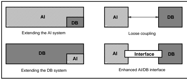
Figure 1: Of the four alternative approaches to AI/DB integration, the Intelligent Database Interface is an example of an enhanced AI/DB interface.
