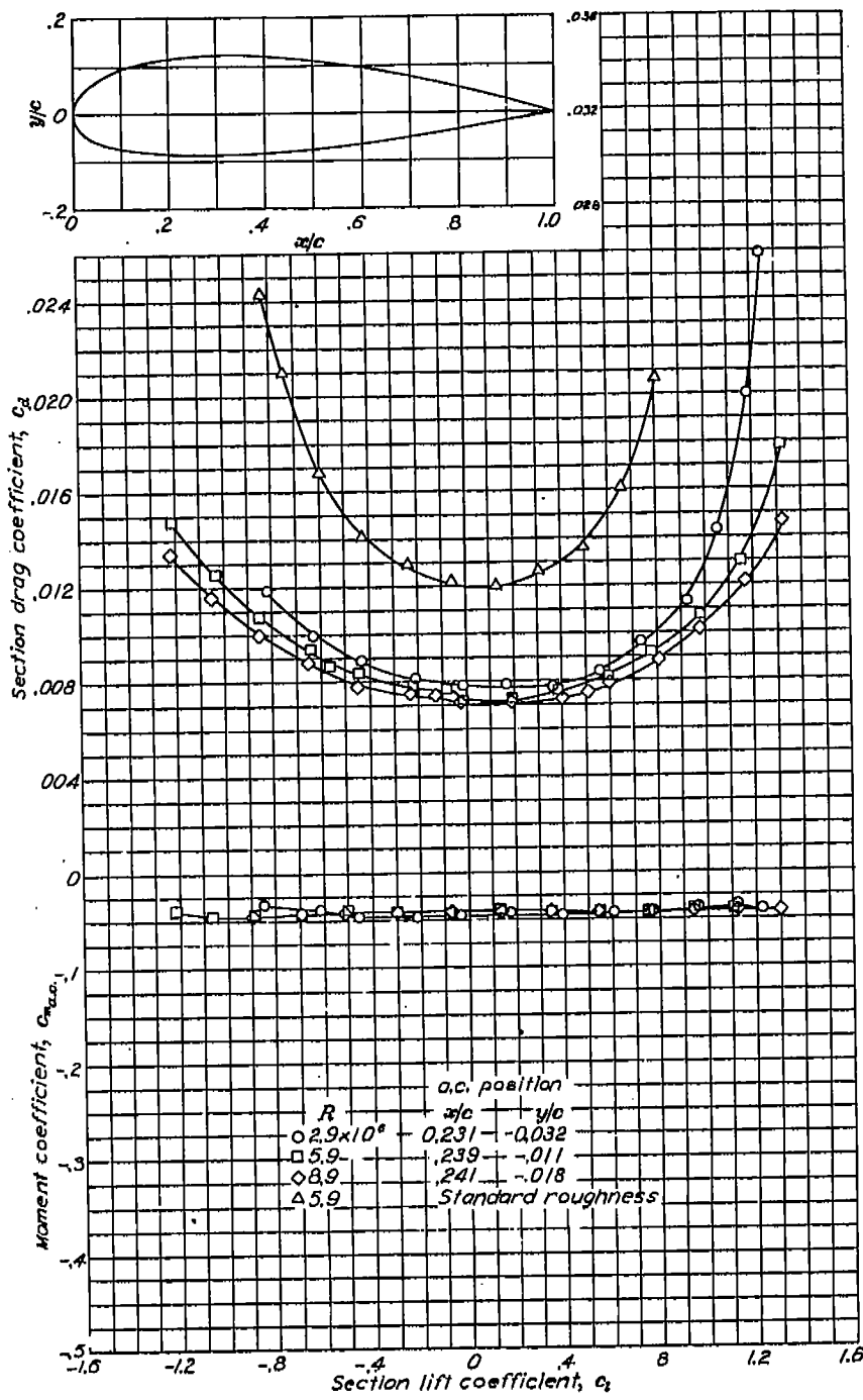
Aerodynamic characteristics of the NACA 2421 airfoil section, 24-inch chord.
