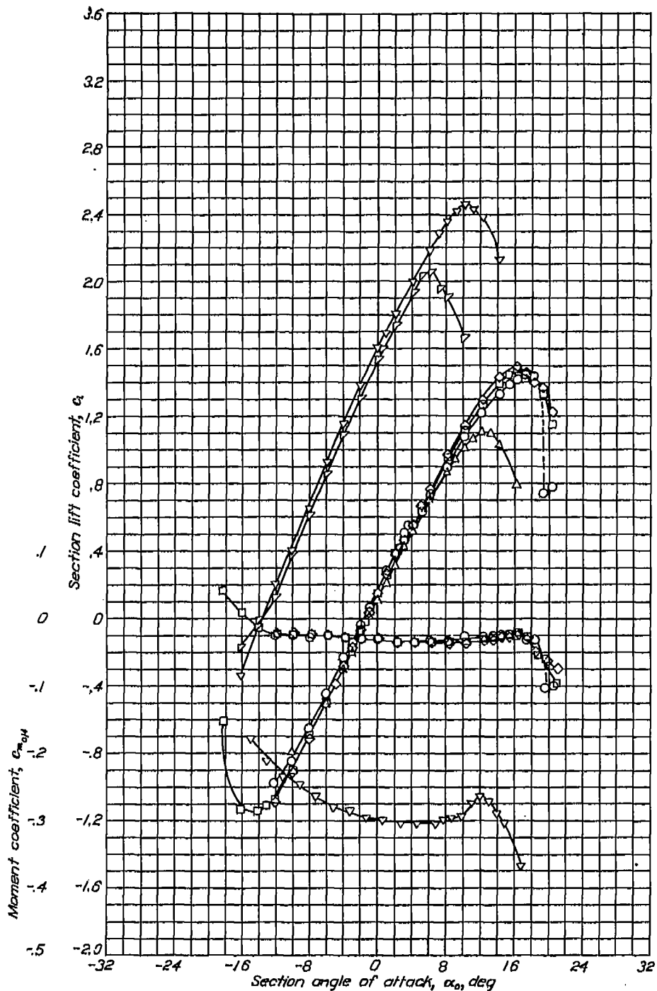
Aerodynamic characteristics of the NACA 662-215 airfoil section, 24-inch chord.
