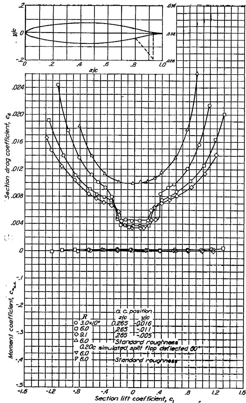
Aerodynamic characteristics of the NACA 66-015 airfoil section, 24-inch chord.
