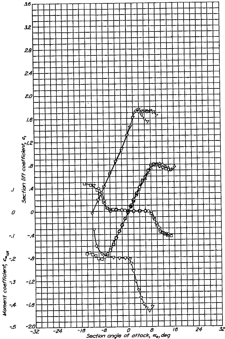
Aerodynamic characteristics of the NACA 00-006 airfoil section, 24-inch chord.
