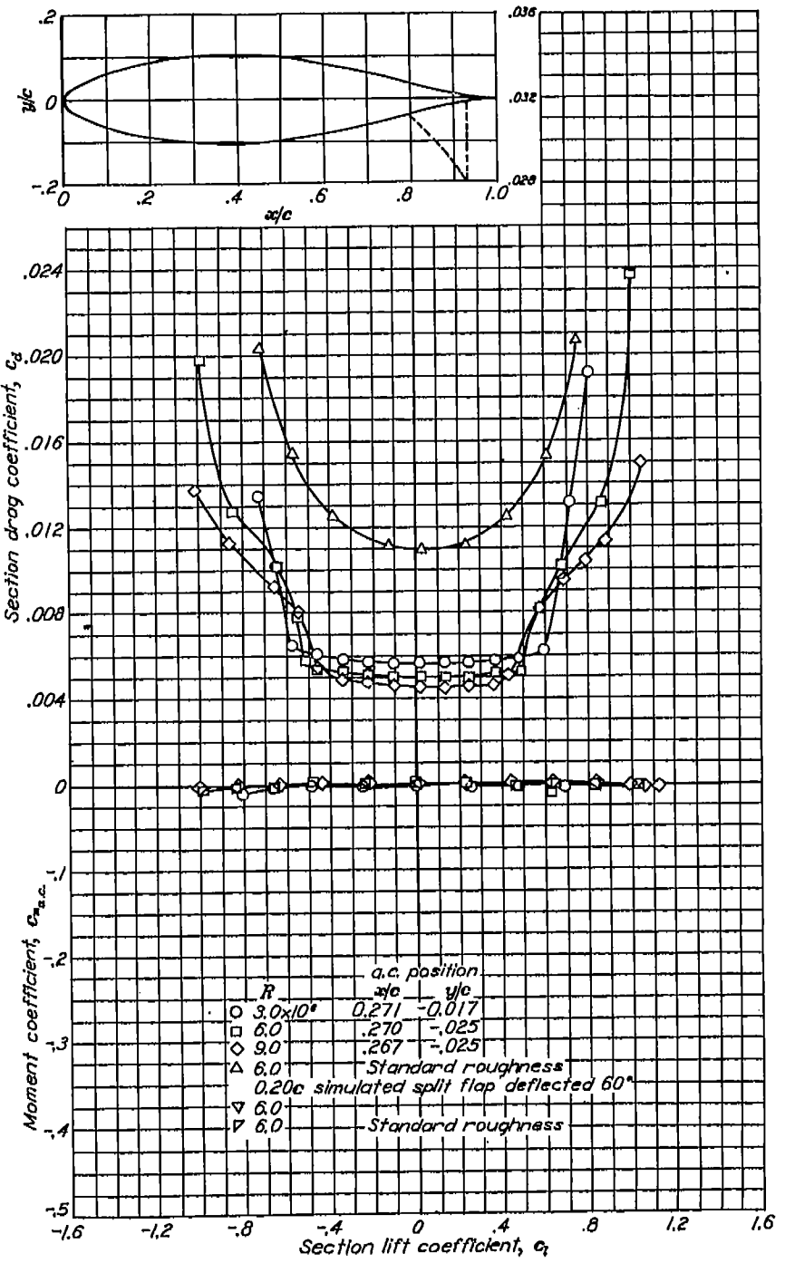
Aerodynamic characteristics of the NACA 65-021 airfoil section, 24-inch chord.
