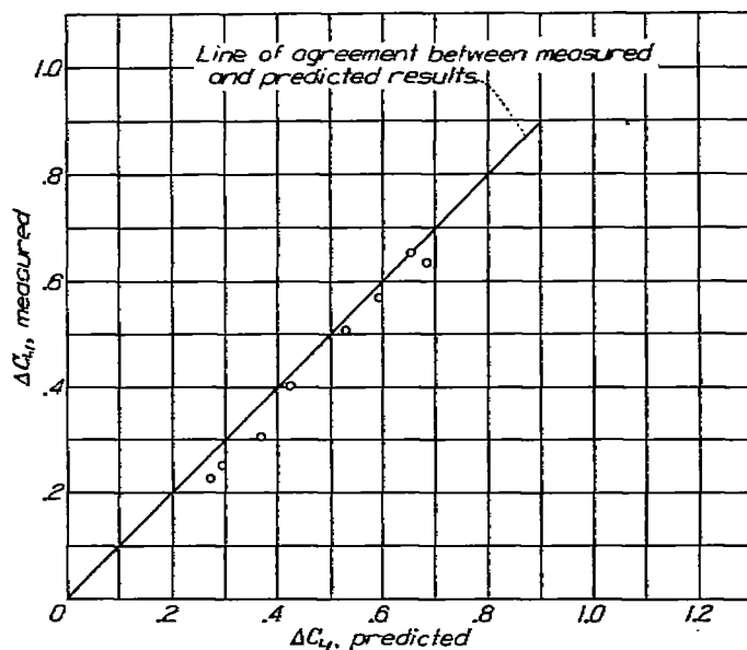
FIGURE 87.—Comparison between measured values of the increments in lift coefficients due to flap deflection and values predicted from two-dimensional data. Split flap.
