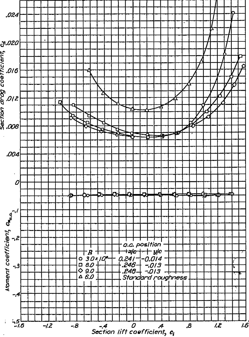
Aerodynamic characteristics of the NACA 2415 airfoil section, 24-inch chord.
