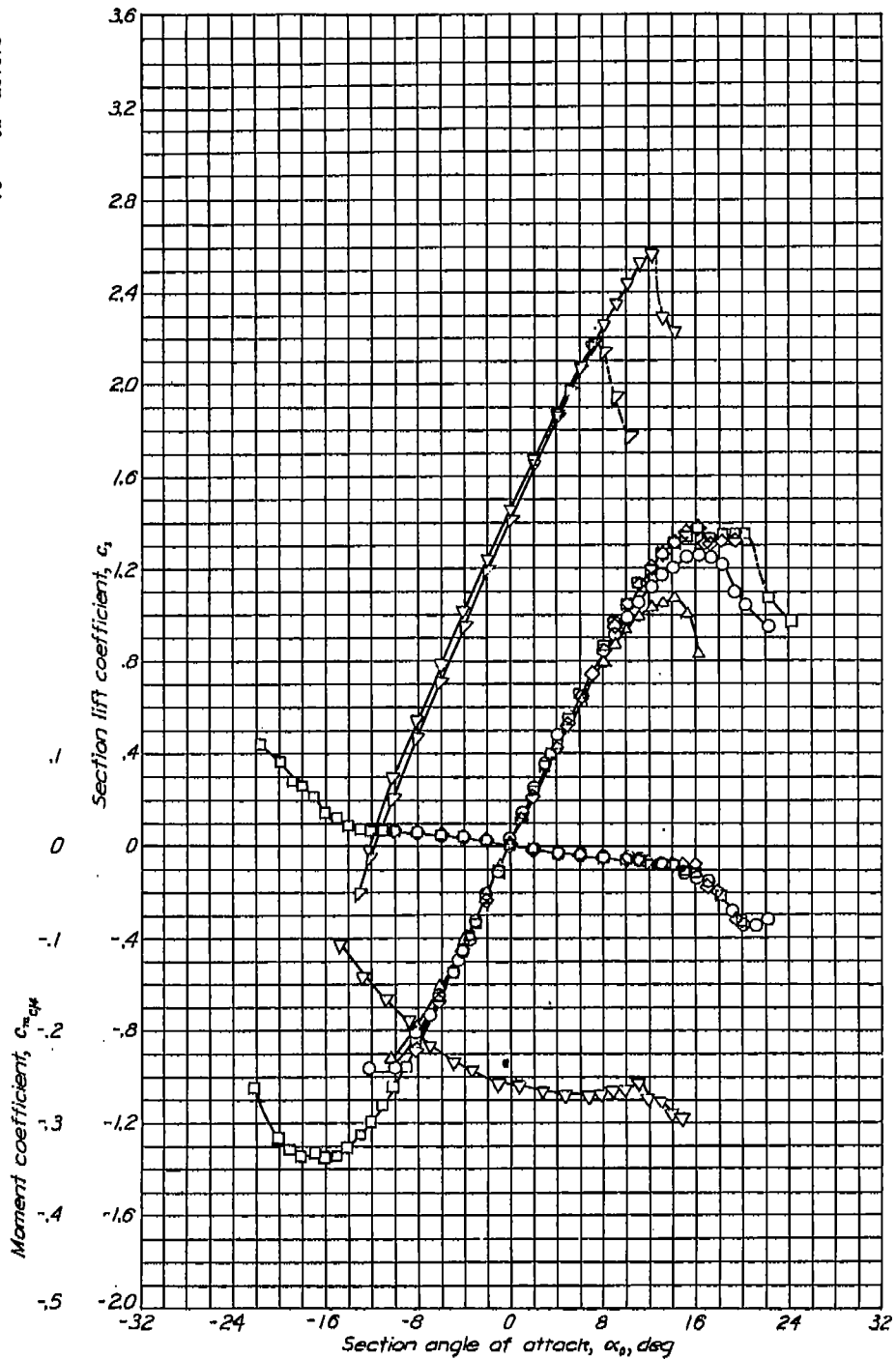
Aerodynamic characteristics of the NACA 65-018 airfoil section, 24-inch chord.
