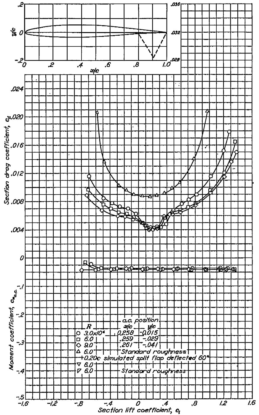
Aerodynamic characteristics of the NACA 64-209 airfoil section, 24-inch chord.
