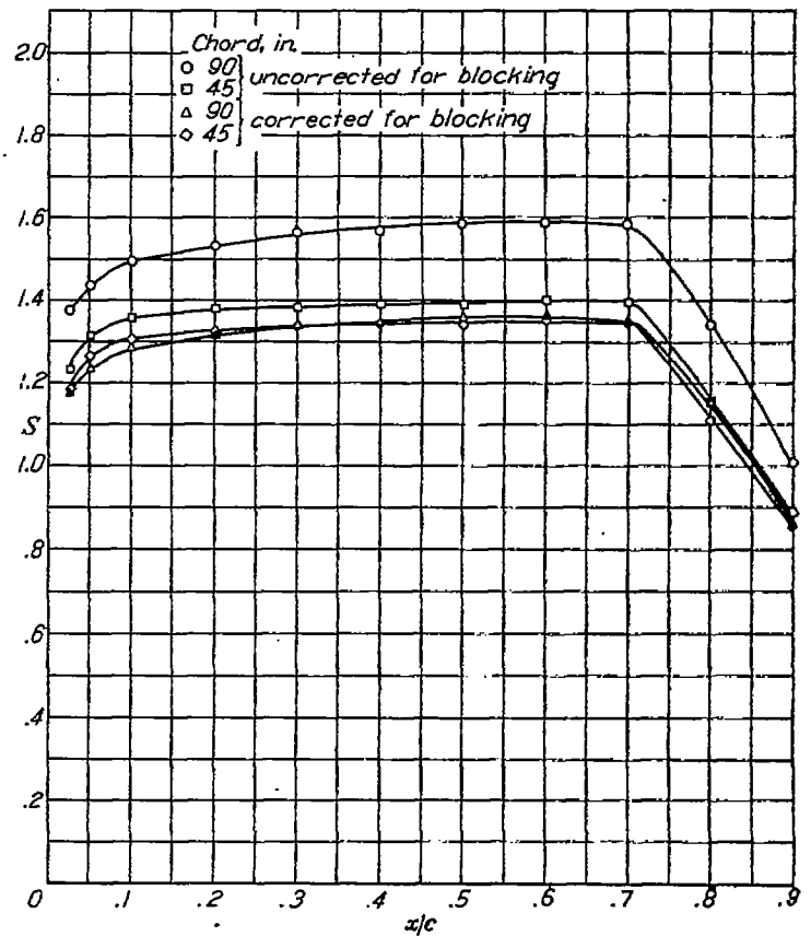
FIGURE 71.—Comparison between corrected and uncorrected pressure distributions for two chord sizes of a symmetrical NACA 6-series airfoil of 15-percent thickness. \alpha_o = 0^\circ
