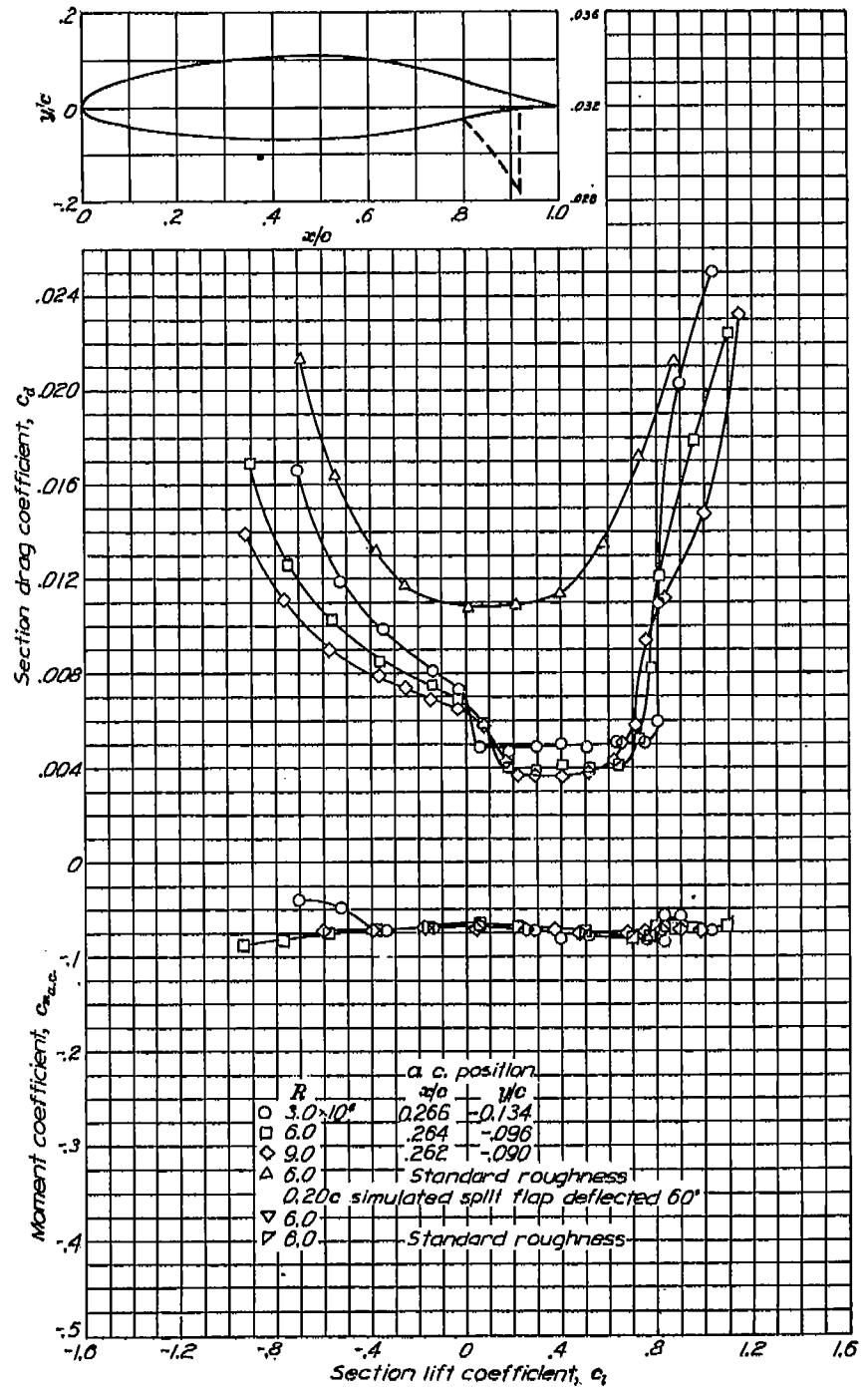
Aerodynamic characteristics of the NACA 66-418 airfoil section, 24-inch chord.
