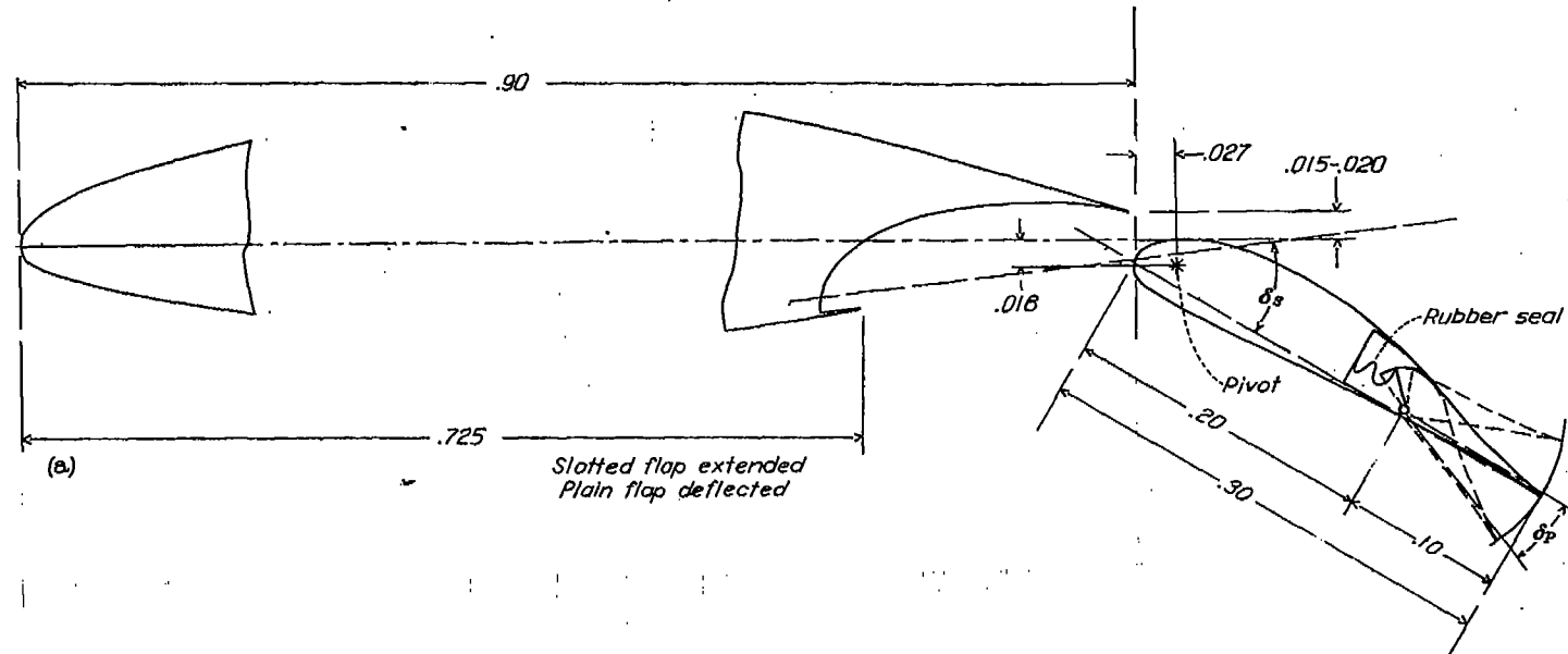
(a) Airfoil-flap configuration.
