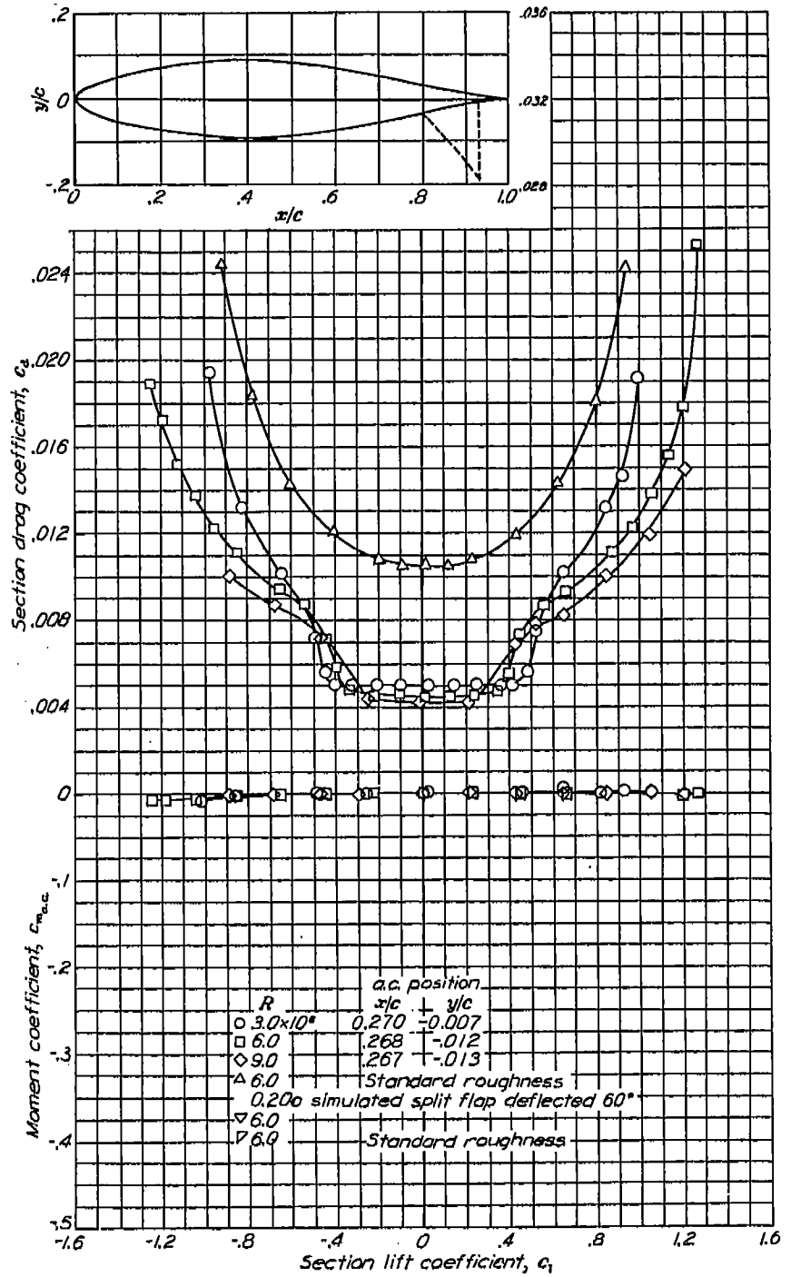
Aerodynamic characteristics of the NACA 65-018 airfoil section, 24-inch chord.
