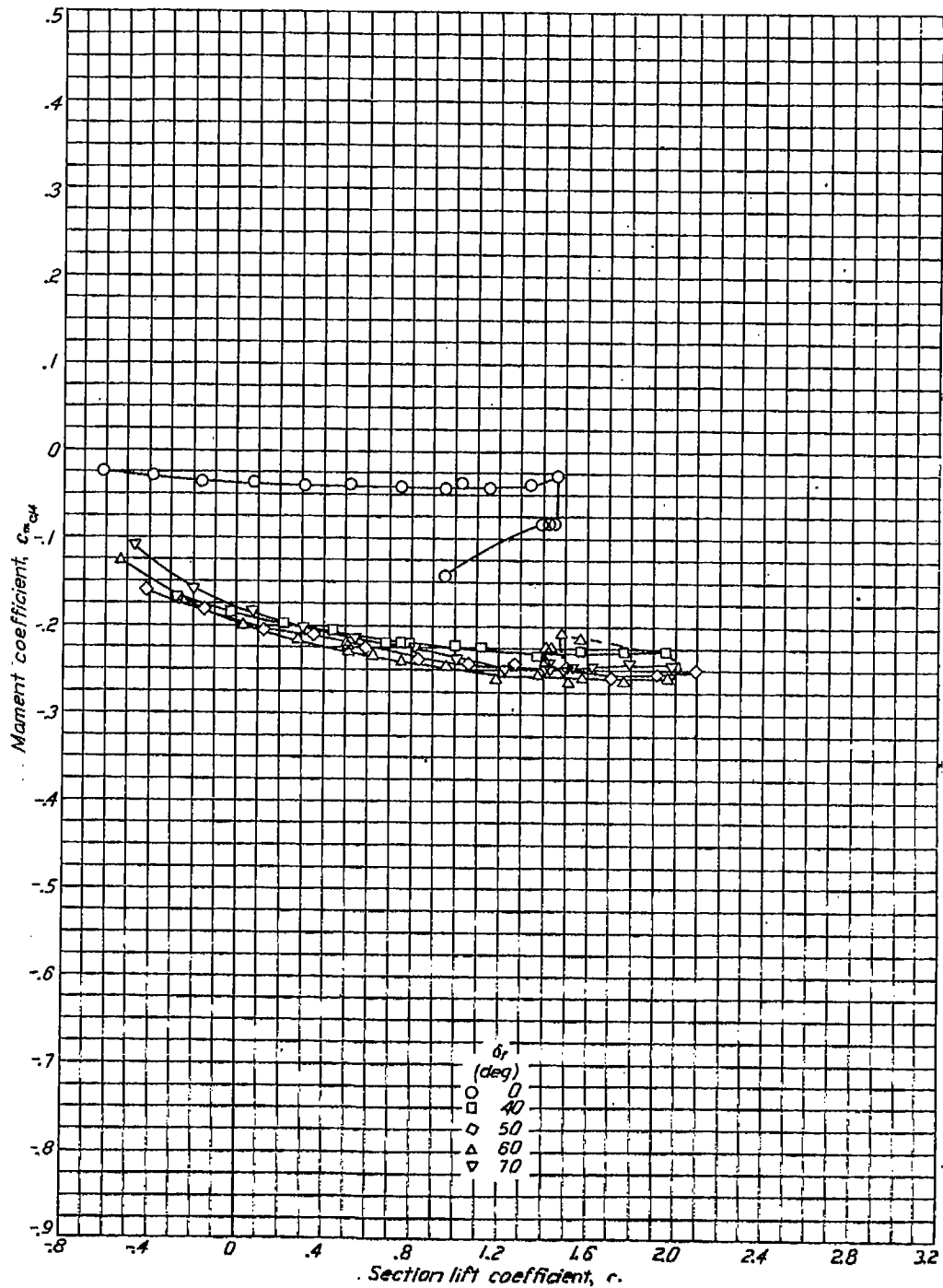
Lift and moment characteristics of the NACA 65-212 airfoil section with 0.20c split flap. R=5 \times 10^6 .
