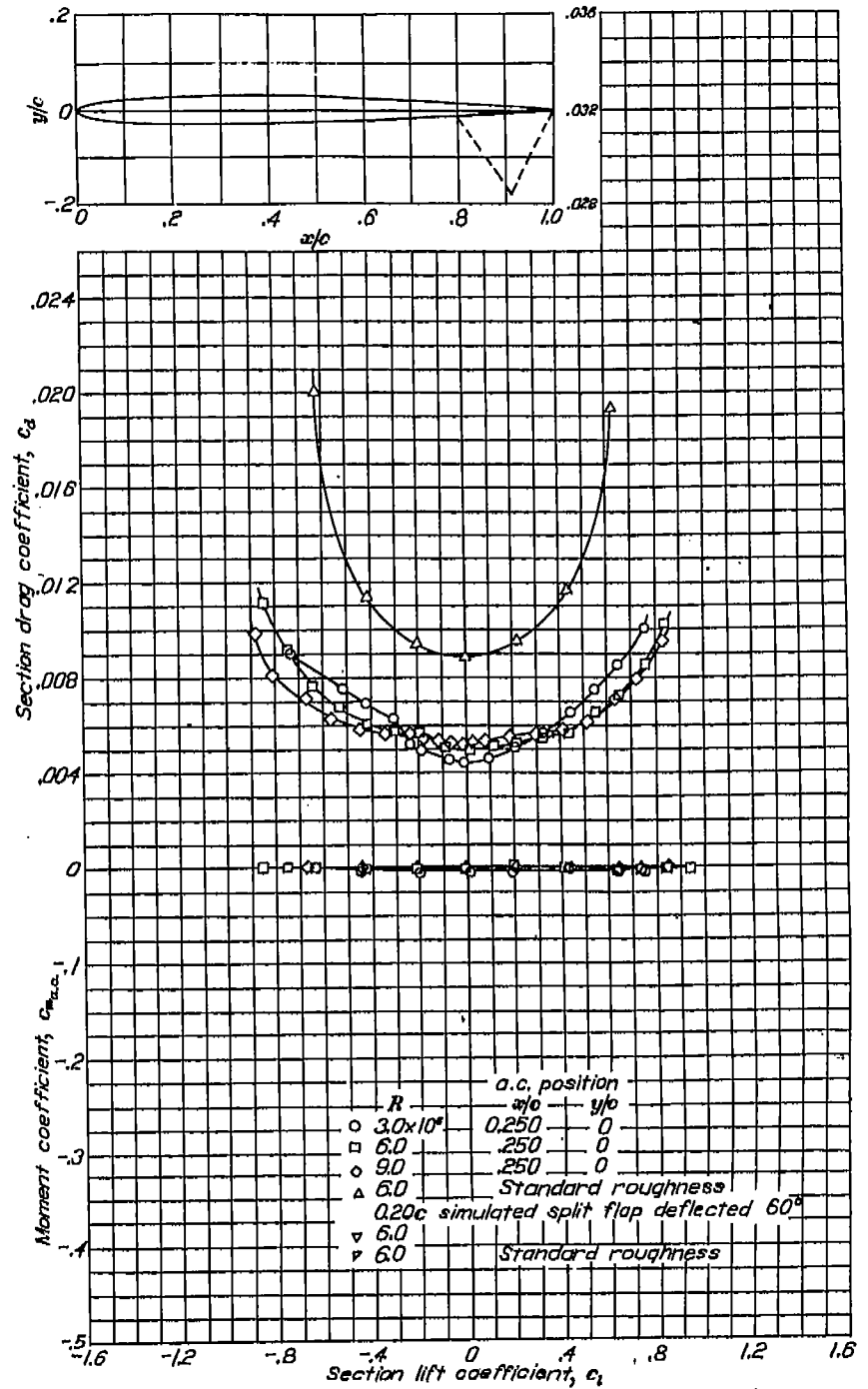
Aerodynamic characteristics of the NACA 0006 airfoil section, 24-inch chord.
