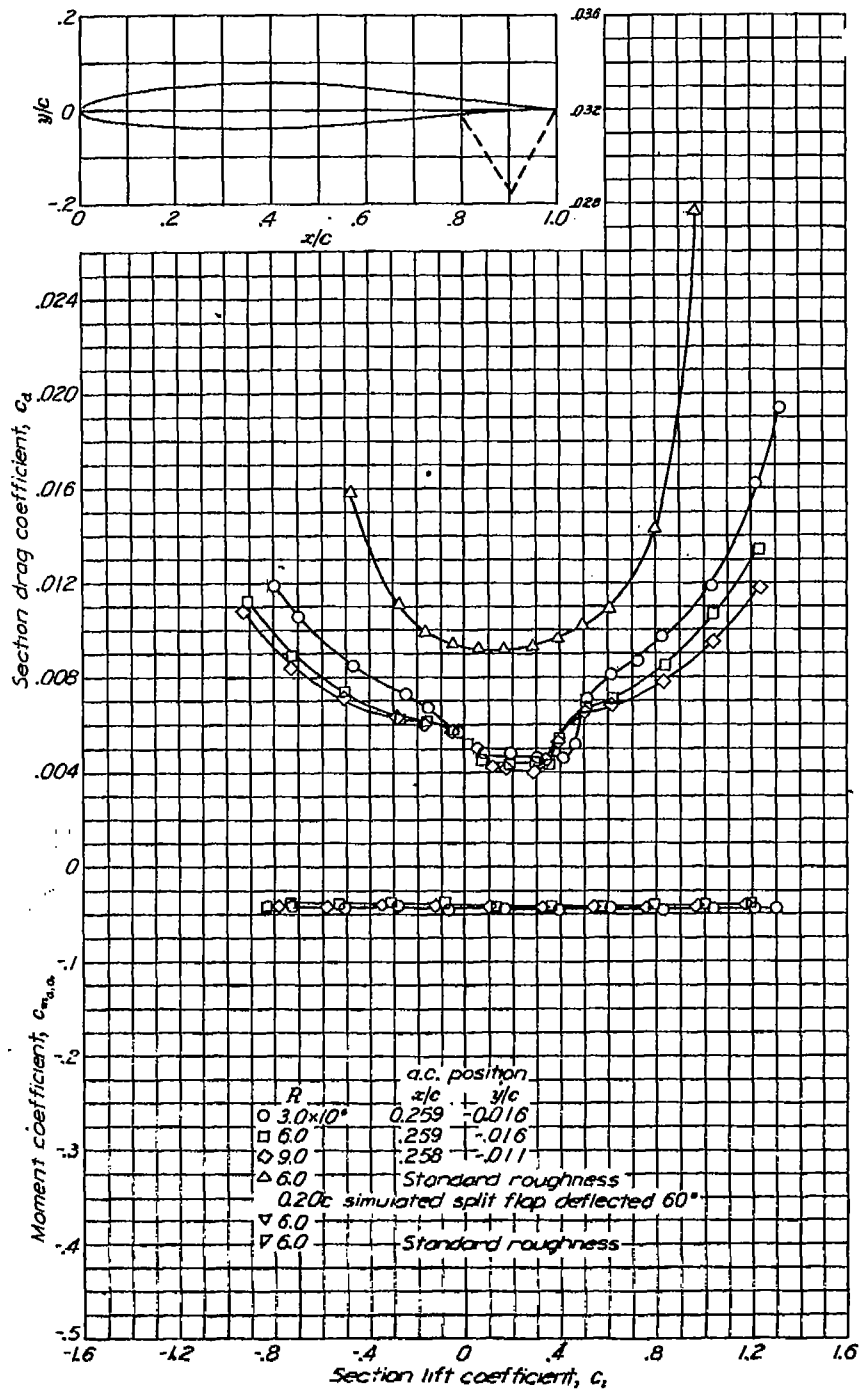
Aerodynamic characteristics of the NACA 64-210 airfoil section, 24-inch chord.
