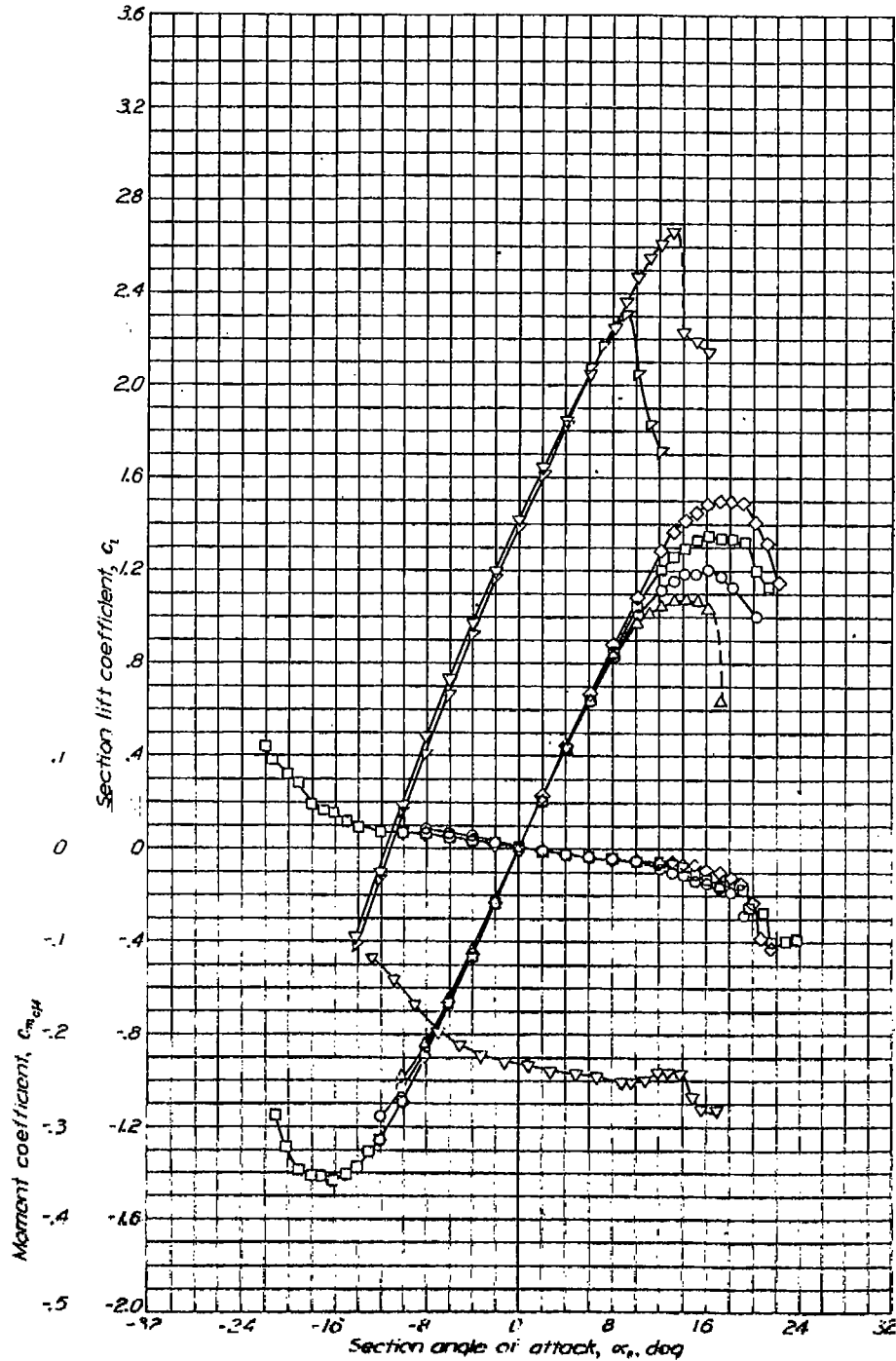
Aerodynamic characteristics of the NACA 64-018 airfoil section, 24-inch chord.
