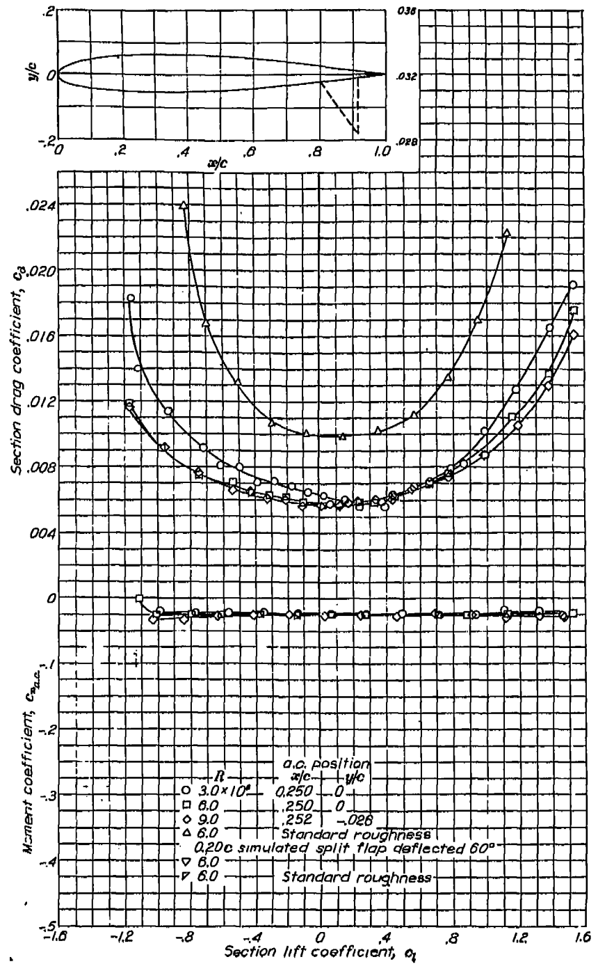
Aerodynamic characteristics of the NACA 1413 airfoil section, 24-inch chord.
