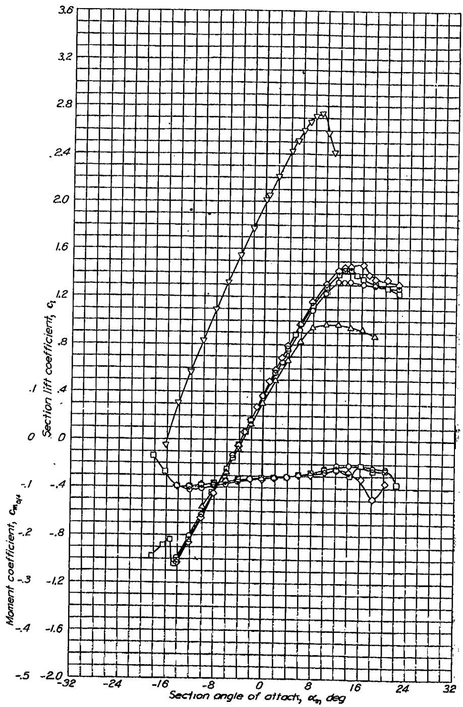
Aerodynamic characteristics of the NACA 4421 airfoil section, 24-inch chord.
