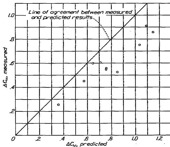
FIGURE 88.—Comparison between measured values of the increments in lift coefficients due to flap deflection and values predicted from two-dimensional data. Slotted flap.
