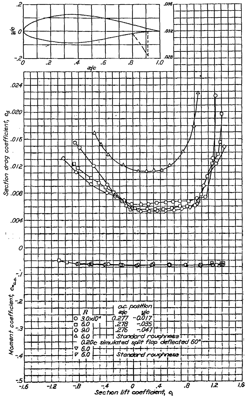
Aerodynamic characteristics of the NACA 64-421 airfoil section, 24-inch chord.
