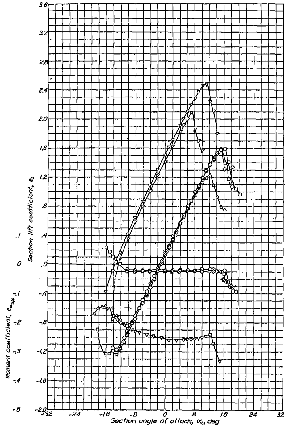
Aerodynamic characteristics of the NACA 1413 airfoil section, 24-inch chord.
