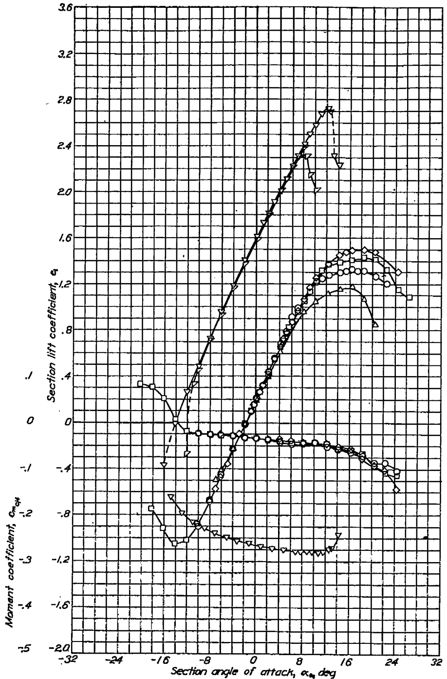
Aerodynamic characteristics of the NACA 747A415 airfoil section, 24-inch chord.
