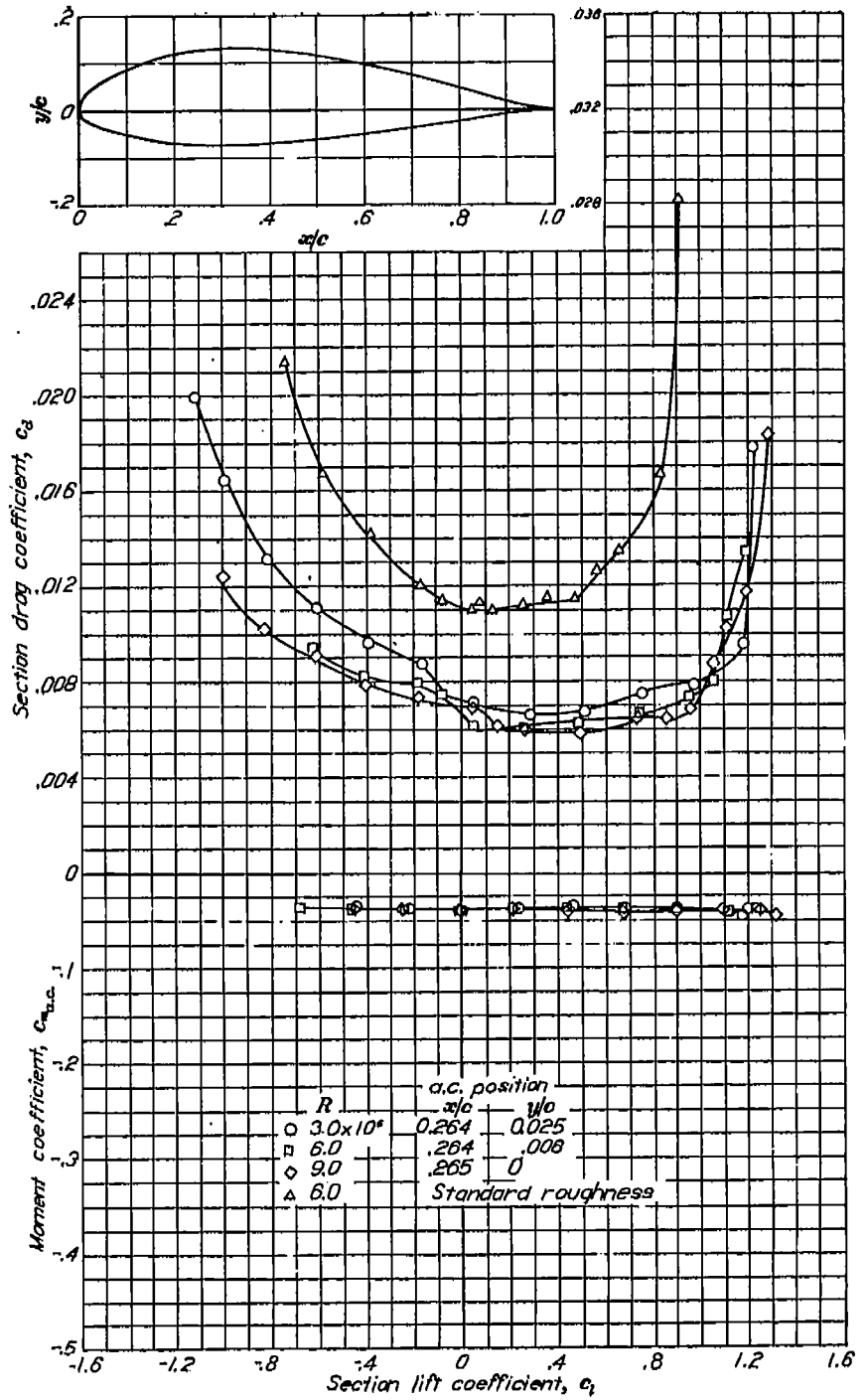
Aerodynamic characteristics of the NACA 63,4-420, a = 0.3 airfoil section, 24-inch chord.
