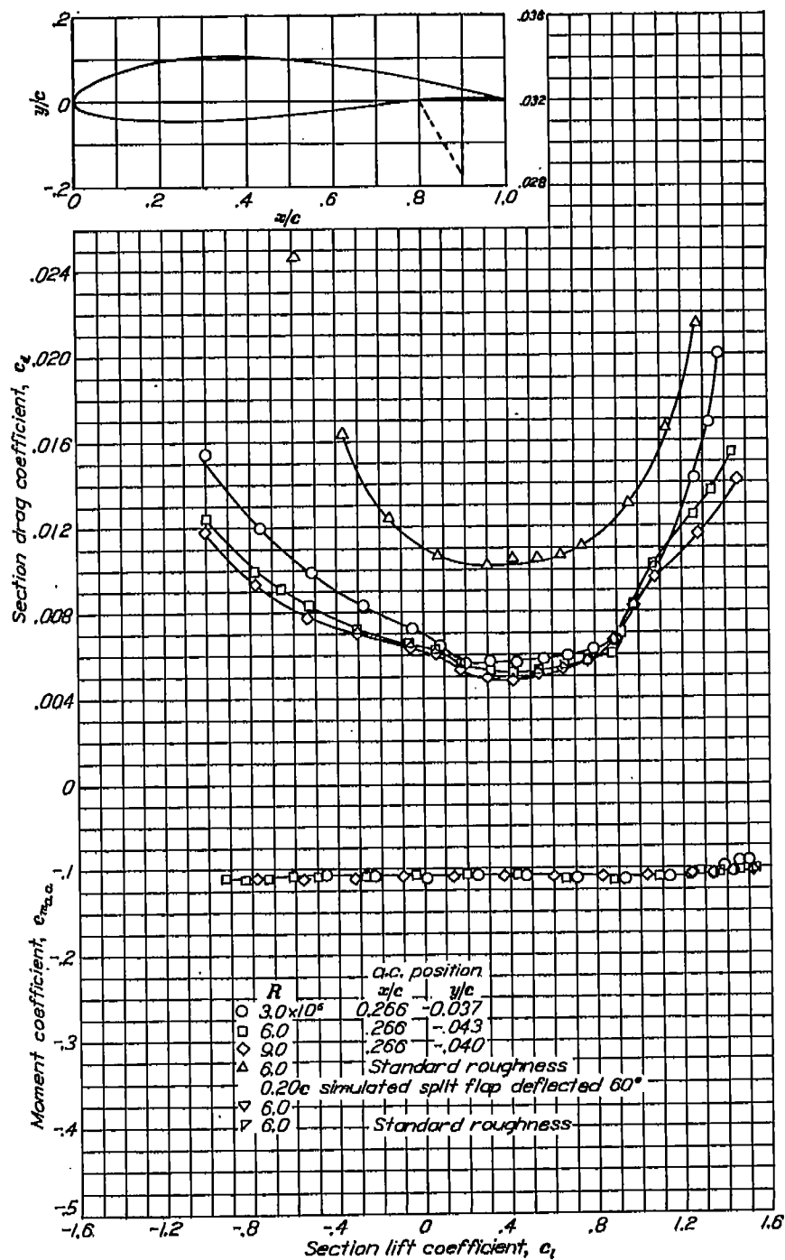
Aerodynamic characteristics of the NACA 632-615 airfoil section, 24-inch chord.
