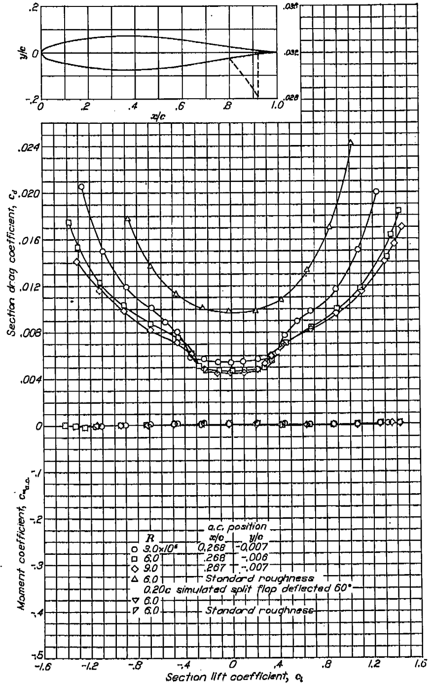
Aerodynamic characteristics of the NACA 642-015 airfoil section, 24-inch chord.
