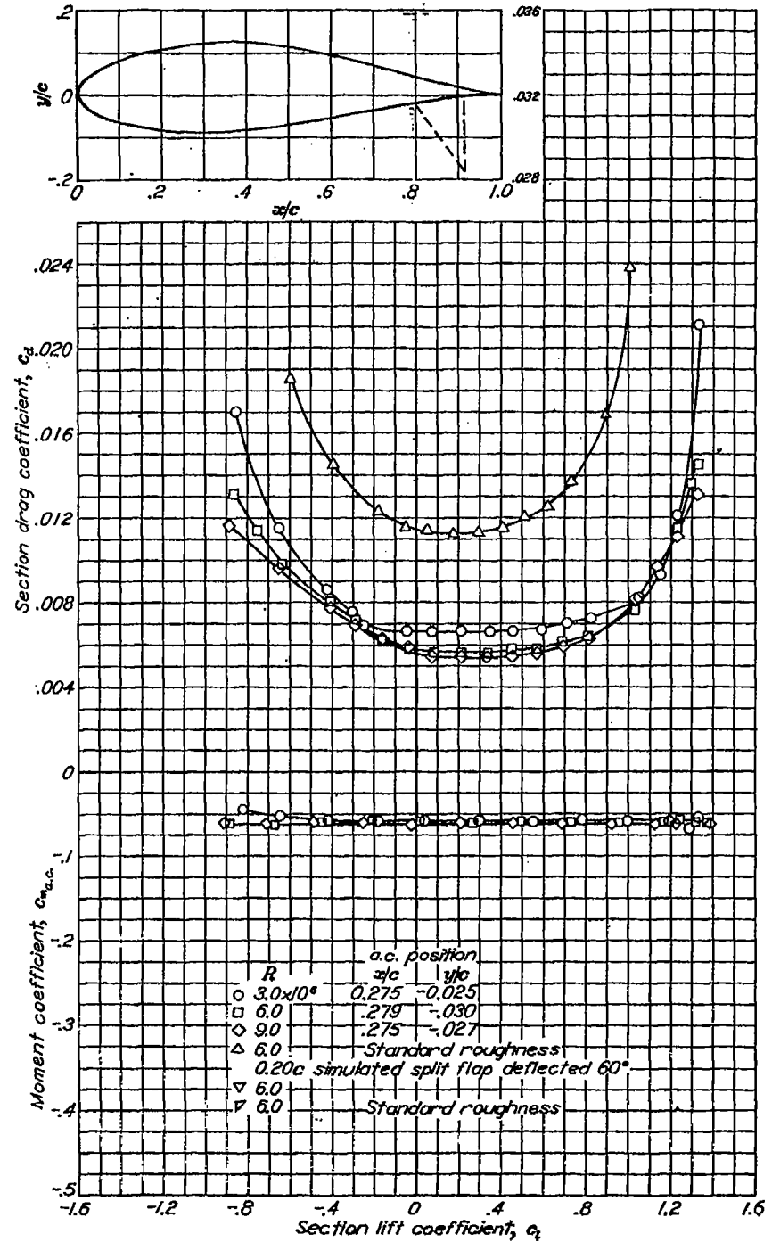
Aerodynamic characteristics of the NACA 63-421 airfoil section, 24-inch chord.
