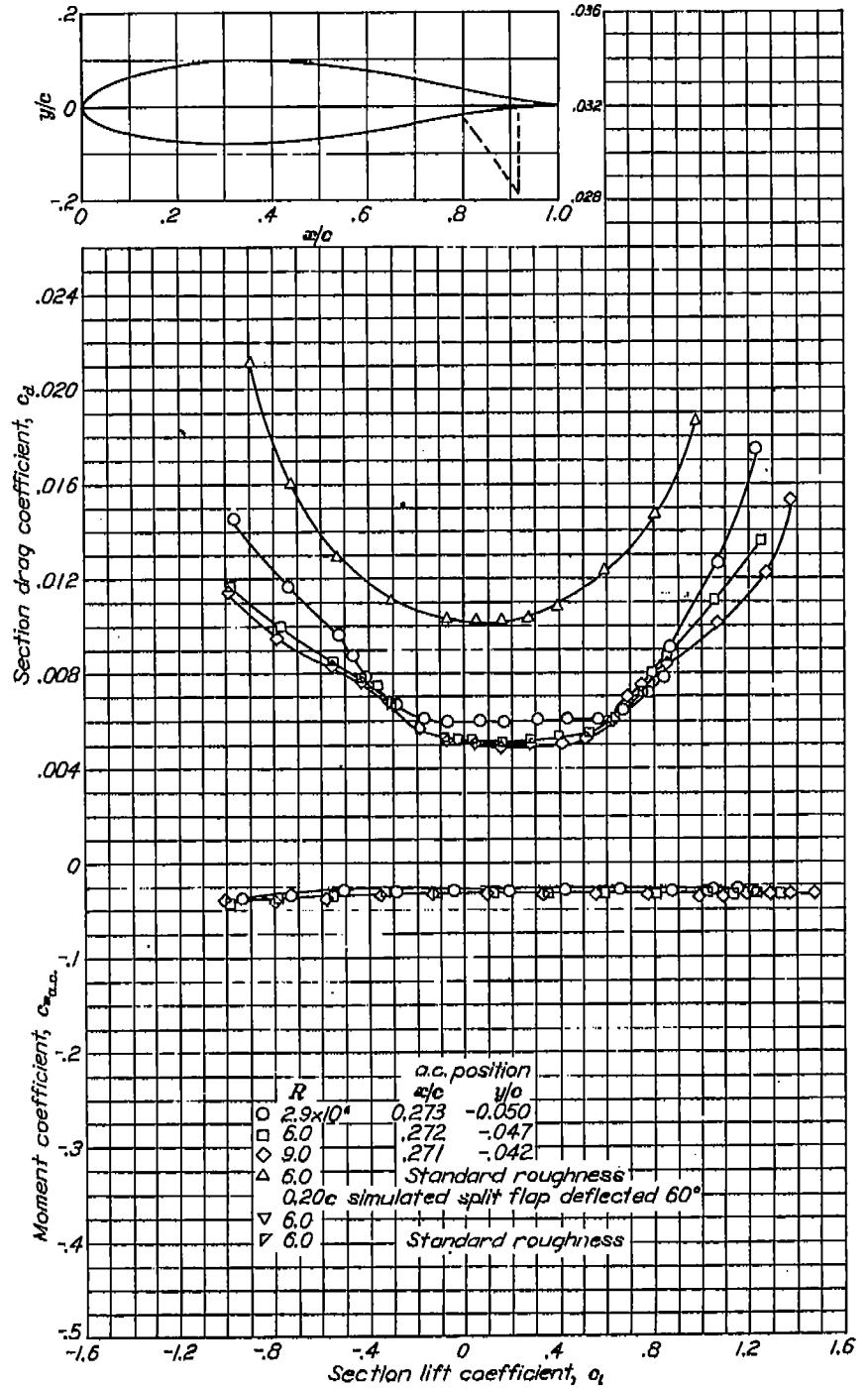
Aerodynamic characteristics of the NACA 633-218 airfoil section, 24-inch chord.
