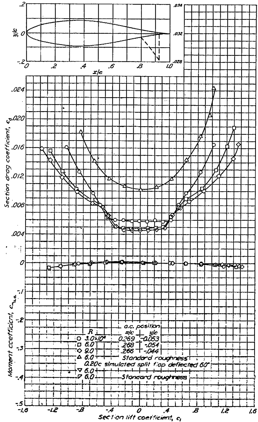
Aerodynamic characteristics of the NACA 64-018 airfoil section, 24-inch chord.
