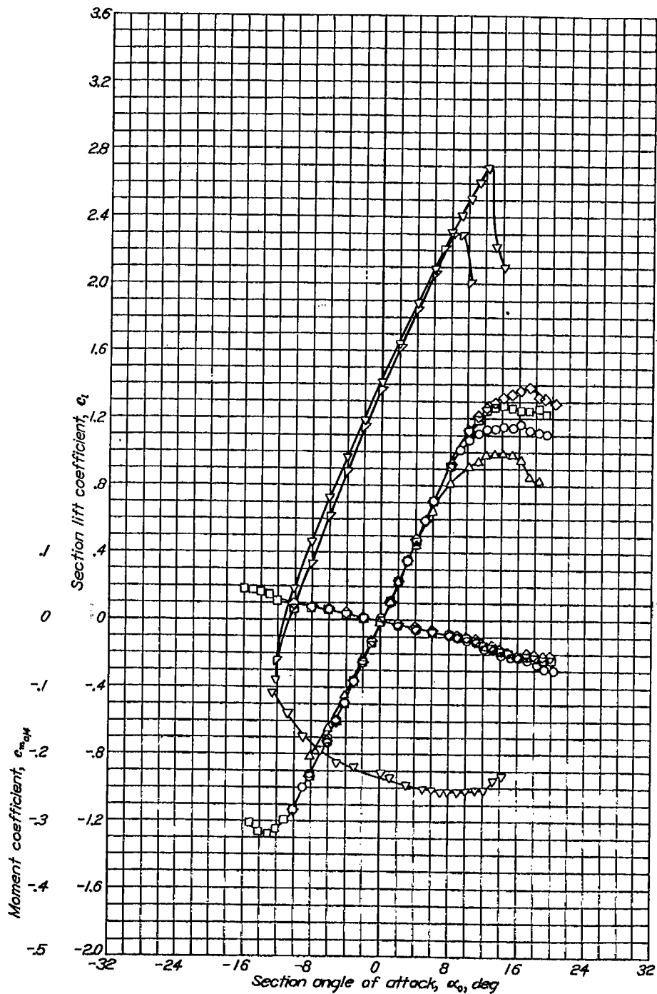
Aerodynamic characteristics of the NACA 63-021 airfoil section, 24-inch chord.
