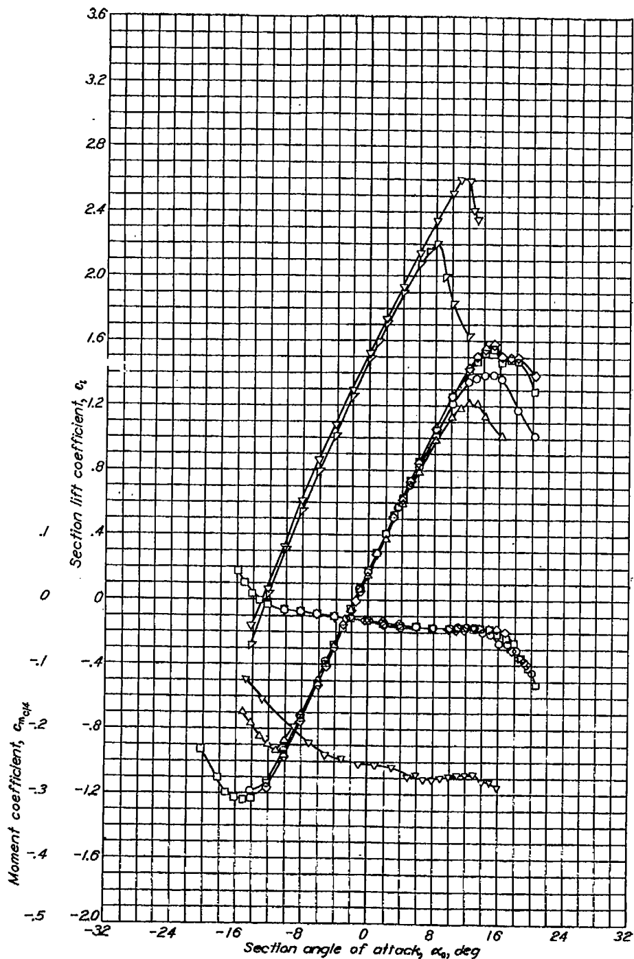
Aerodynamic characteristics of the NACA 64-215 airfoil section, 24-inch chord.
