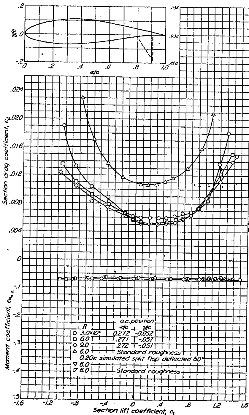
Aerodynamic characteristics of the NACA 63-418 airfoil section, 24-inch chord.
