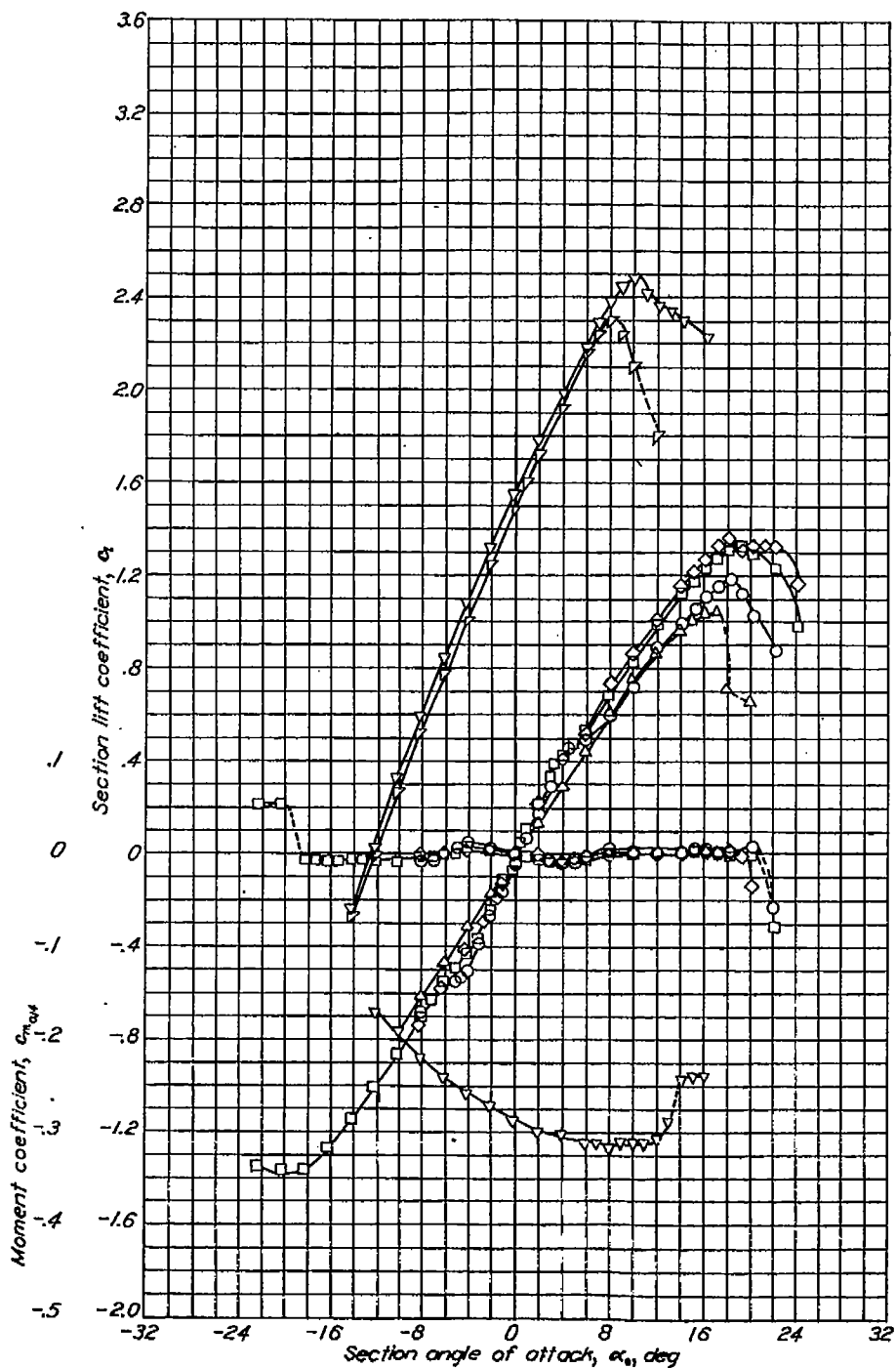
Aerodynamic characteristics of the NACA 664-021 airfoil section, 24-inch chord.
