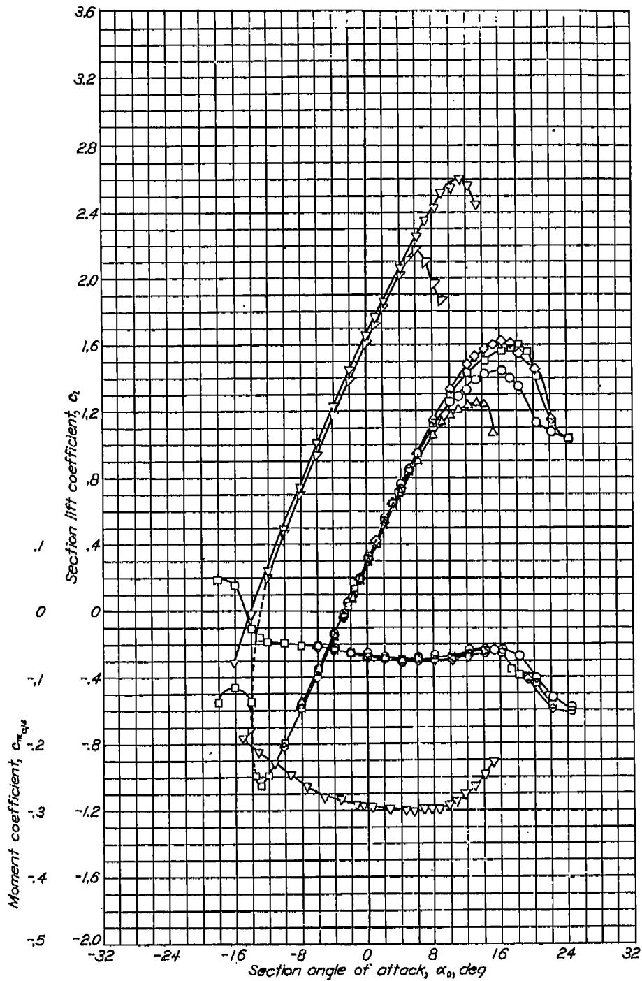
Aerodynamic characteristics of the NACA 06-415 airfoil section, 24-inch chord.
