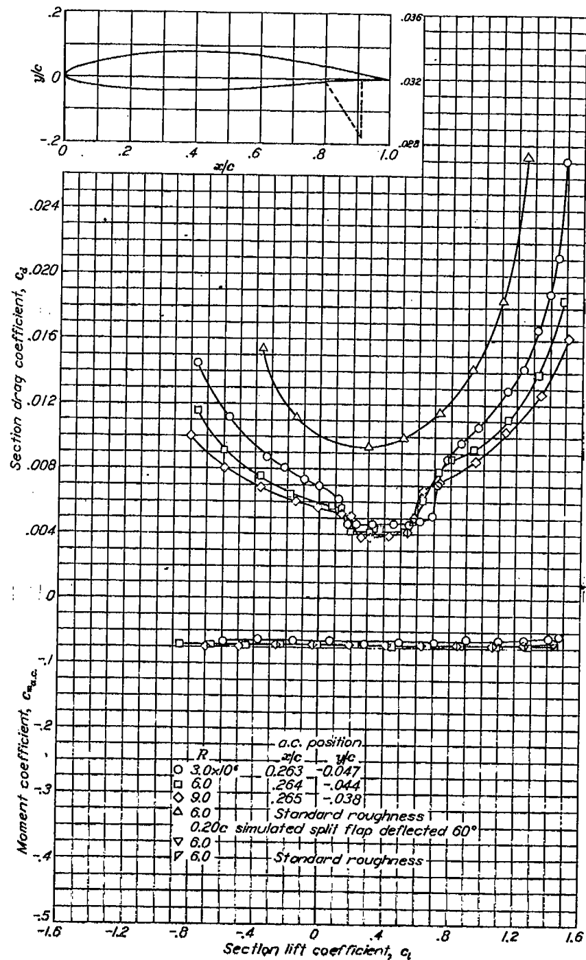
Aerodynamic characteristics of the NACA 65-112 airfoil section, 24-inch chord.
