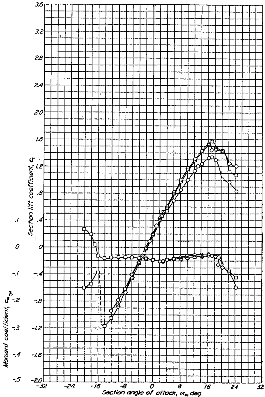
Aerodynamic characteristics of the NACA 66(215)-216 airfoil section, 21-inch chord.
