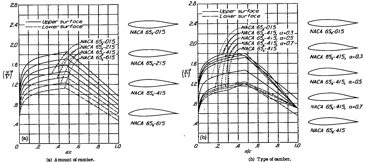
FIGURE 8.—Effect of amount and type of camber on pressure distribution at design lift.
