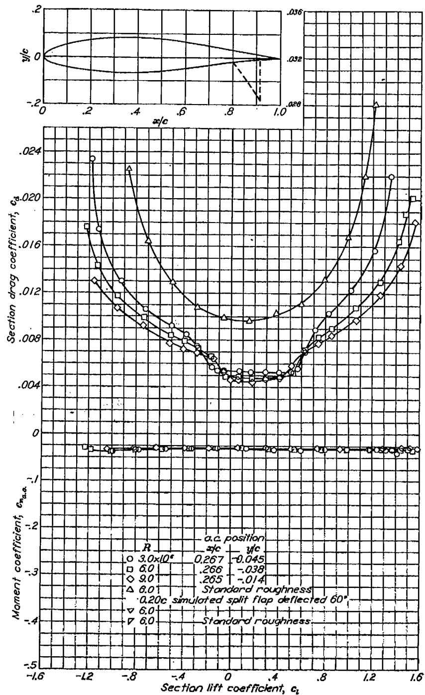
Aerodynamic characteristics of the NACA 64-215 airfoil section, 24-inch chord.
