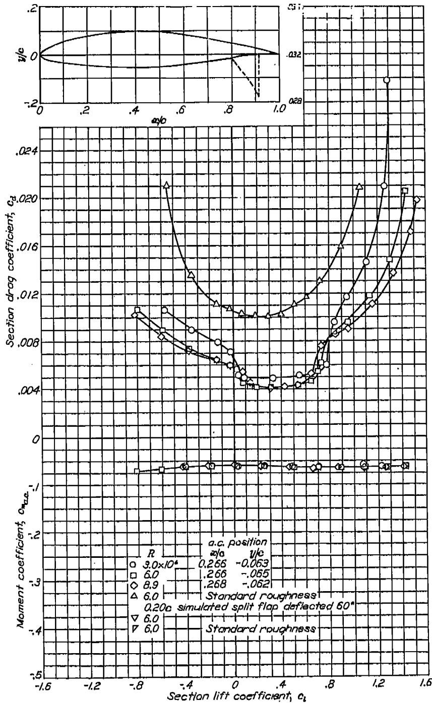
Aerodynamic characteristics of the NACA 06-415 airfoil section, 24-inch chord.
