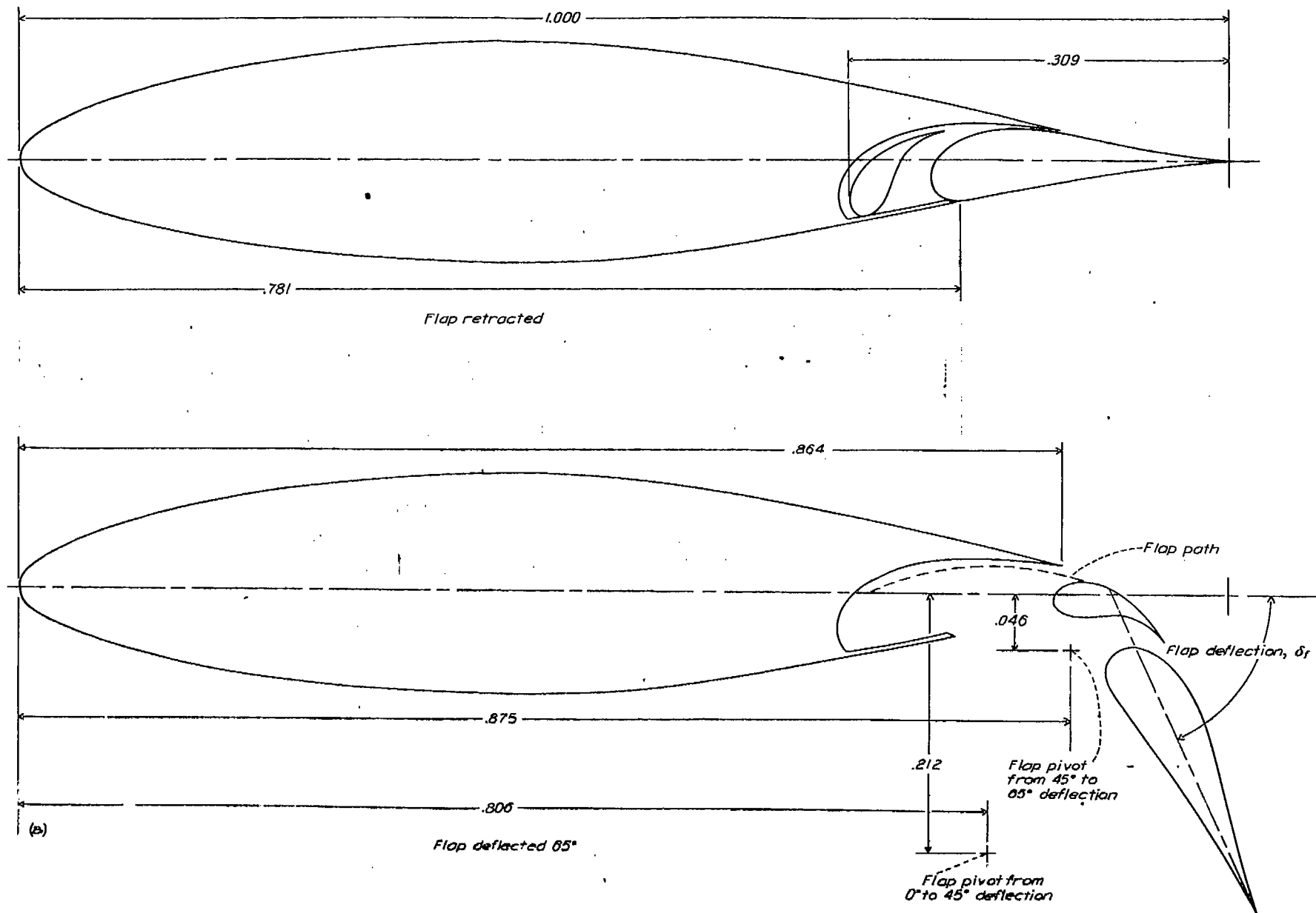
(a) Configuration. NACA 65-118 airfoil section with 0.309 double slotted flap.
