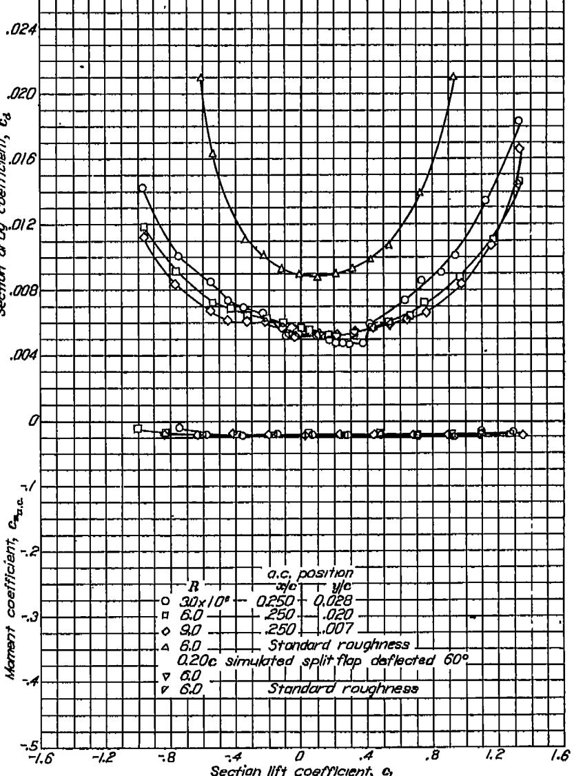
Aerodynamic characteristics of the NACA 1408 airfoil section, 24-inch chord.
