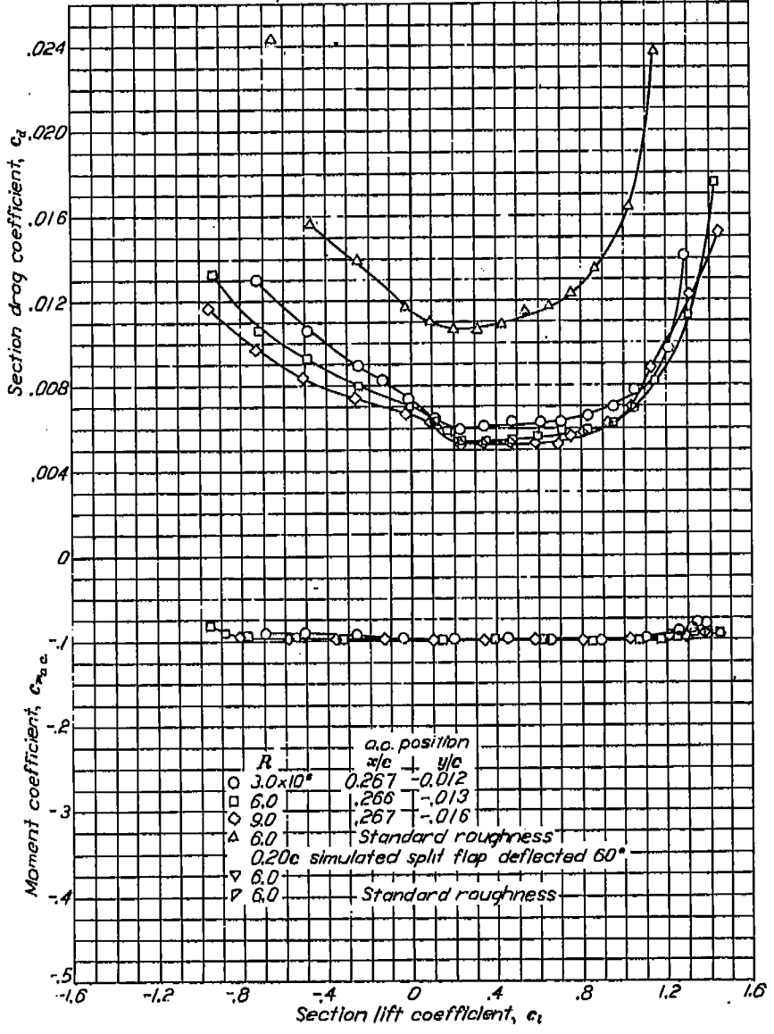
Aerodynamic characteristics of the NACA 63-618 airfoil section, 24-inch chord.
