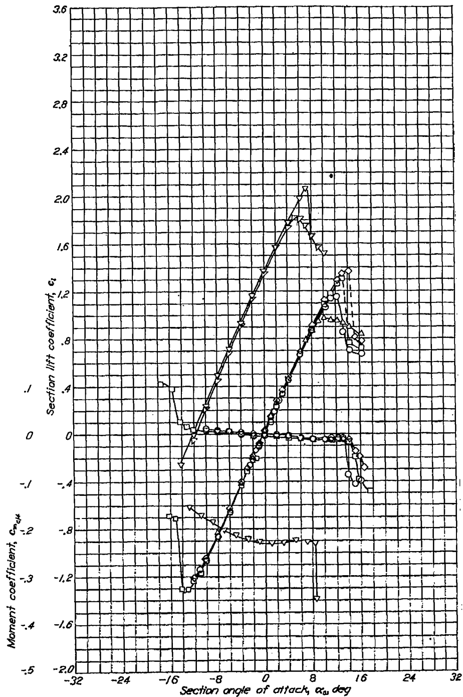
Aerodynamic characteristics of the NACA 65-012 airfoil section, 24-inch chord.
