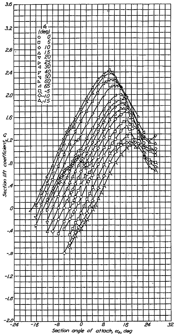
Aerodynamic characteristics of the NACA 66(215)-216 airfoil section with 0.20% sealed plain flap. R=6 \times 10^4 .
