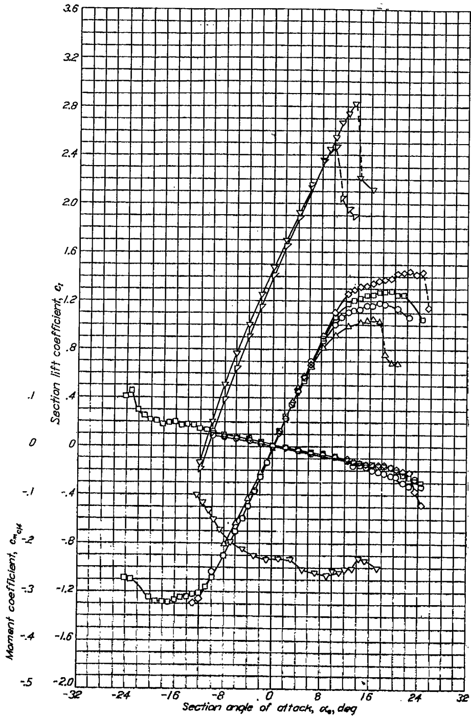
Aerodynamic characteristics of the NACA 644-021 airfoil section, 24-inch chord.
