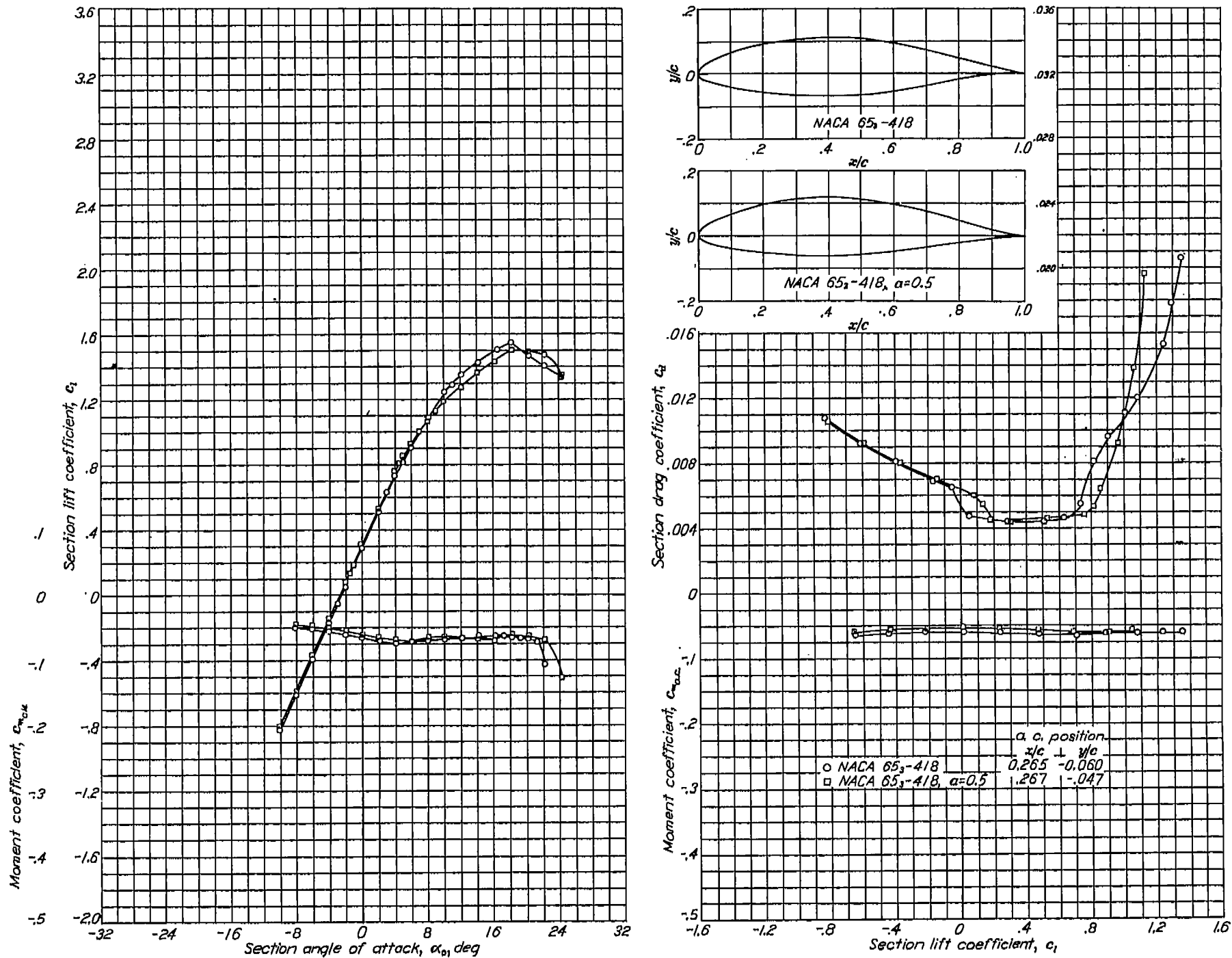
FIGURE 16.—Comparison of the aerodynamic characteristics of the NACA 65 3 -418 and NACA 65 3 -418, \alpha = 0.5 airfoils at a Reynolds number of 9 \times 10^6 . T.D.T. tests 814, 820, 406, and 411.
