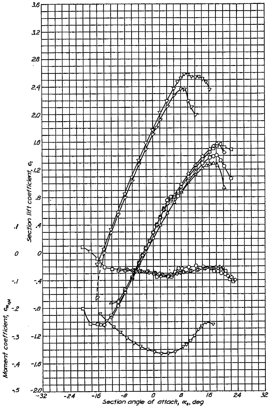
Aerodynamic characteristics of the NACA 66-418 airfoil section, 24-inch chord.
