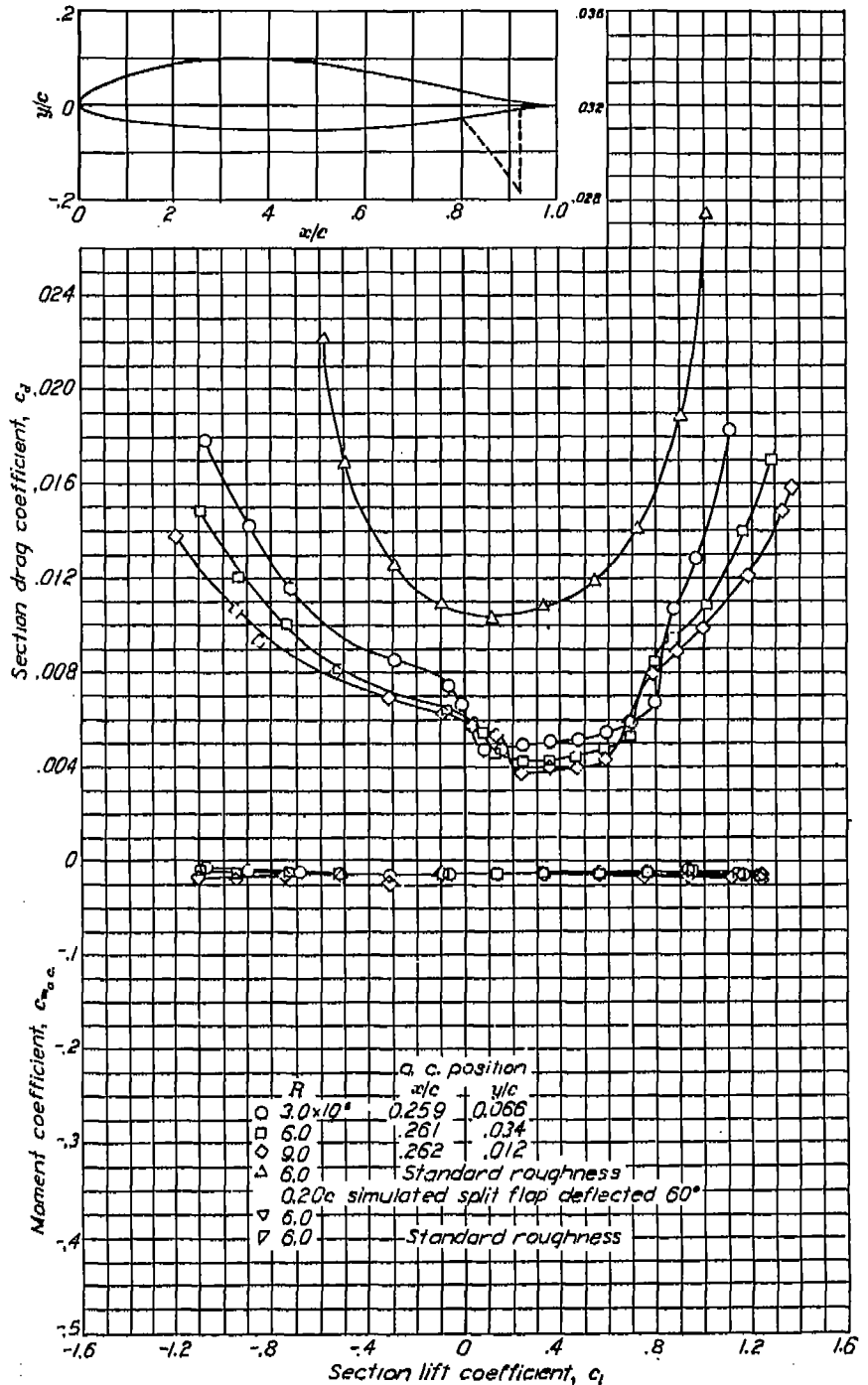
Aerodynamic characteristics of the NACA 747A315 airfoil section, 24-inch chord,
