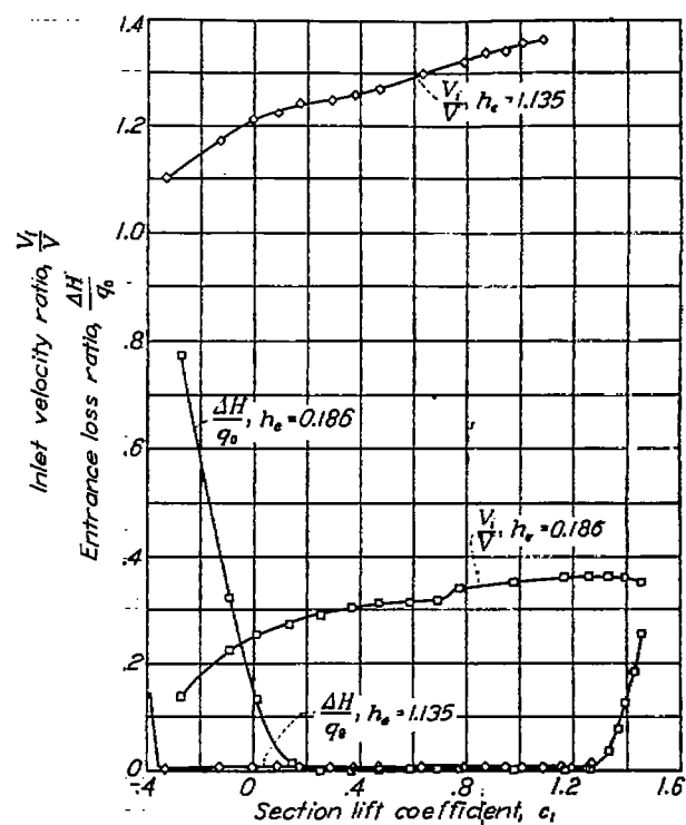
FIGURE 63.—Lift and flow characteristics of an NACA 7-series type airfoil section with leading-edge air intake.
