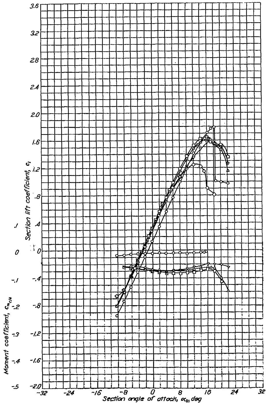
FIGURE 17.—Comparison of the aerodynamic characteristics of some NACA airfoils from tests in the Langley two-dimensional low-turbulence pressure tunnel.
