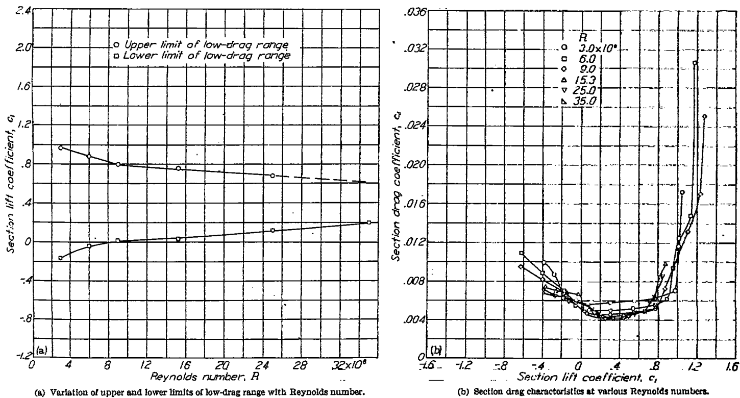
FIGURE 14.—Variation of low-drag range with Reynolds number for the NACA 65(11)-420 airfoil. TDT tests 300, 312, and 322.
