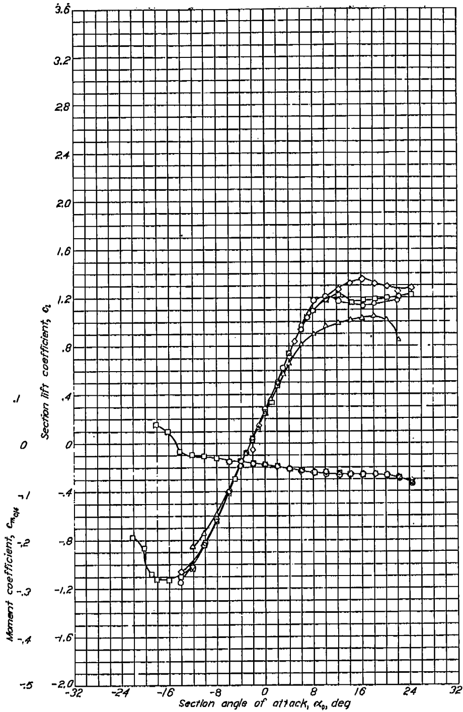
Aerodynamic characteristics of the NACA 63,4-420, a = 0.3 airfoil section, 24-inch chord.
