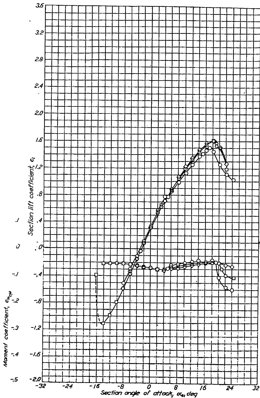
Aerodynamic characteristics of the NACA 66(215)-416 airfoil section, 24-inch chord.
