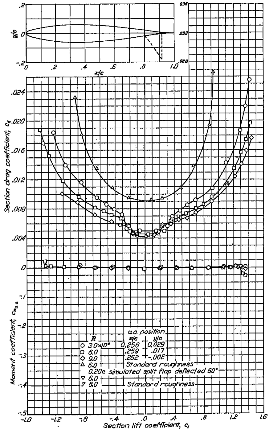
Aerodynamic characteristics of the NACA 64-012 airfoil section, 24-inch chord.
