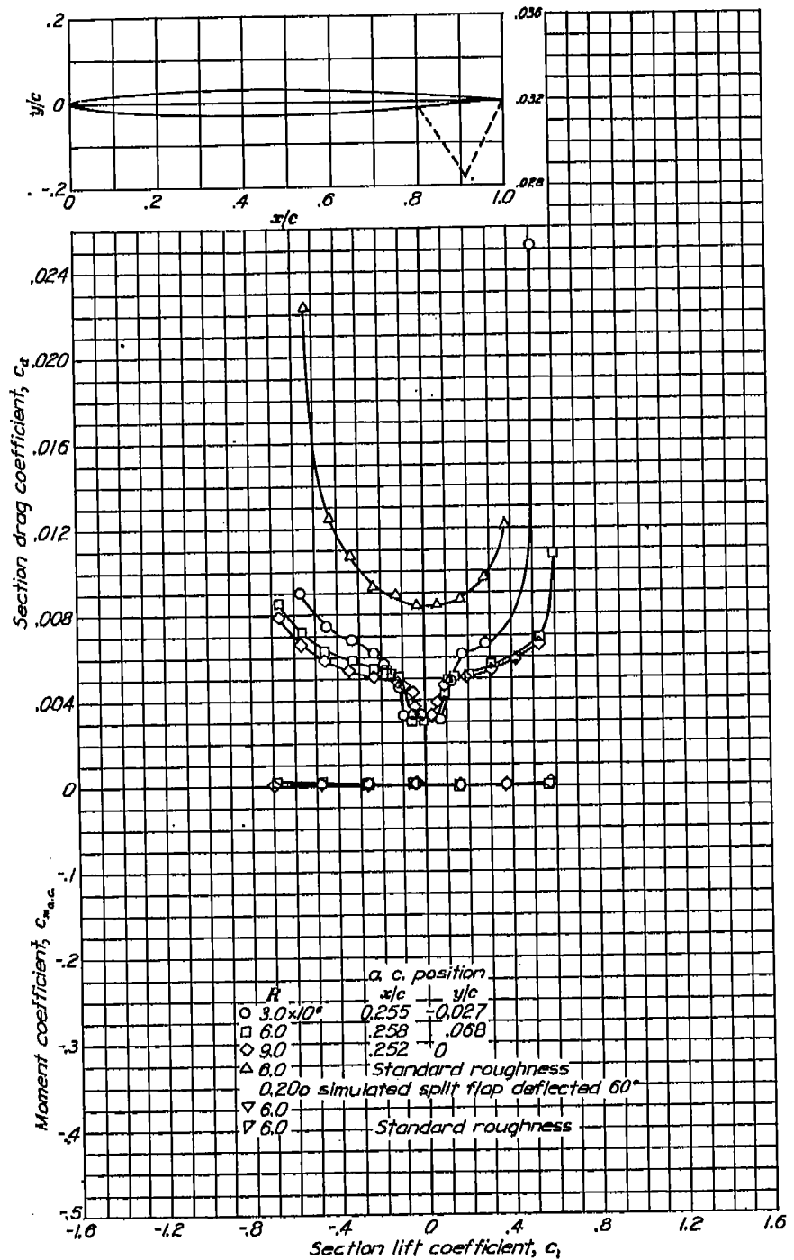
Aerodynamic characteristics of the NACA 00-006 airfoil section, 24-inch chord.
