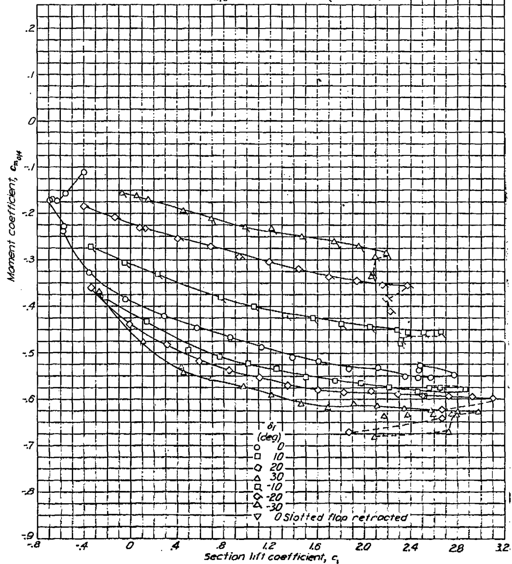
(f) Lift and moment characteristics. Slotted flap deflected 32^\circ ; R=6 \times 10^6 . NACA 66(215)-216, \alpha=0.6 airfoil section with 0.30c slotted and 0.10c plain flap.
