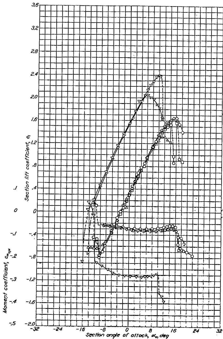
Aerodynamic characteristics of the NACA 65-112 airfoil section, 24-inch chord.
