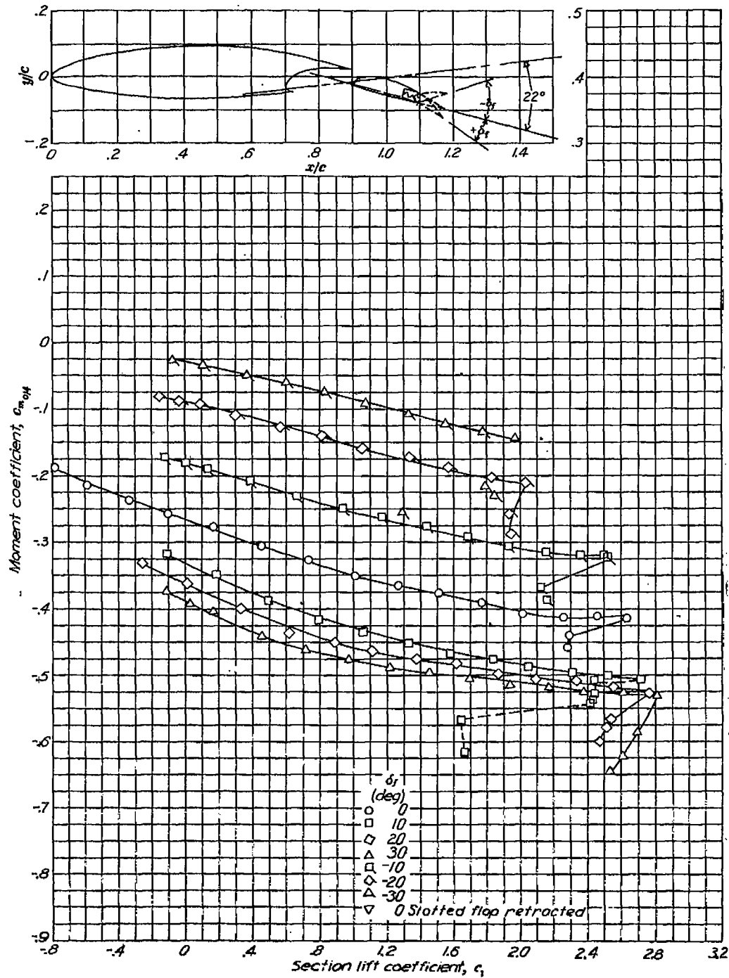
(d) Lift and moment characteristics. Slotted flap deflected 22°; R=6 \times 10^6 . NACA 66(215)-216, a=0.6 airfoil section with 0.30c slotted and 0.10c plain flap.
