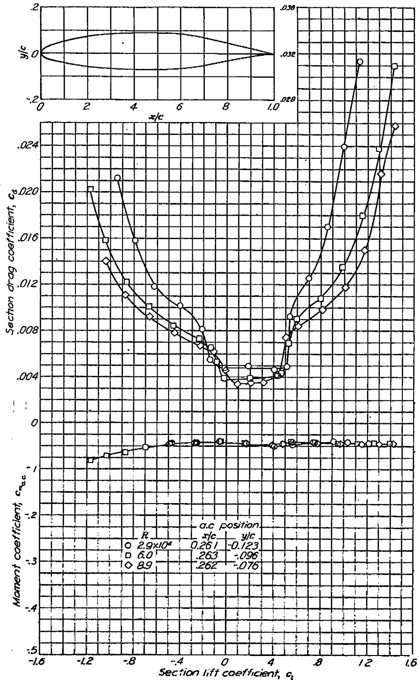
Aerodynamic characteristics of the NACA 66(215)-216 airfoil section, 21-inch chord.
