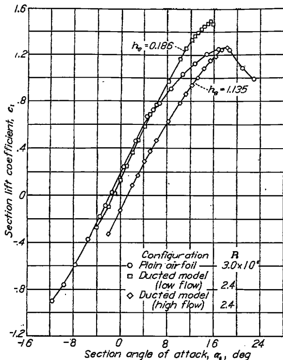
FIGURE 63.—Lift and flow characteristics of an NACA 7-series type airfoil section with leading-edge air intake.
