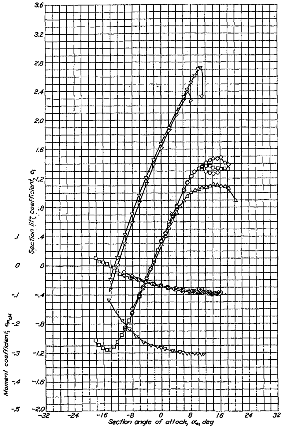
Aerodynamic characteristics of the NACA 63-421 airfoil section, 24-inch chord.
