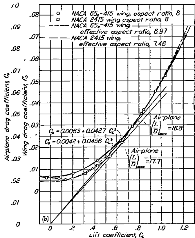
(b) NACA 65-415 and 2415 wings of aspect ratio 8.
