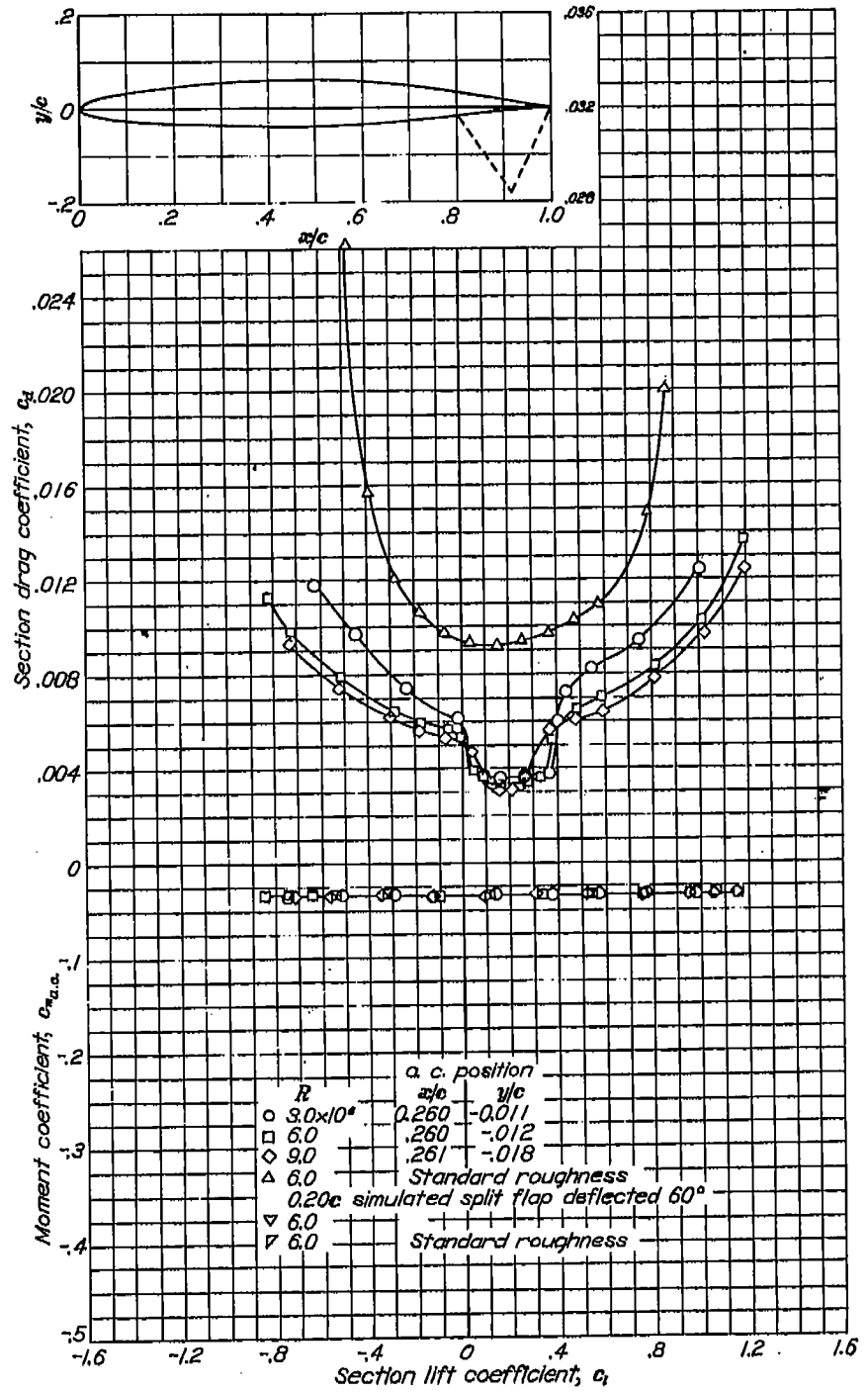
Aerodynamic characteristics of the NACA 66-210 airfoil section, 24-inch chord.
