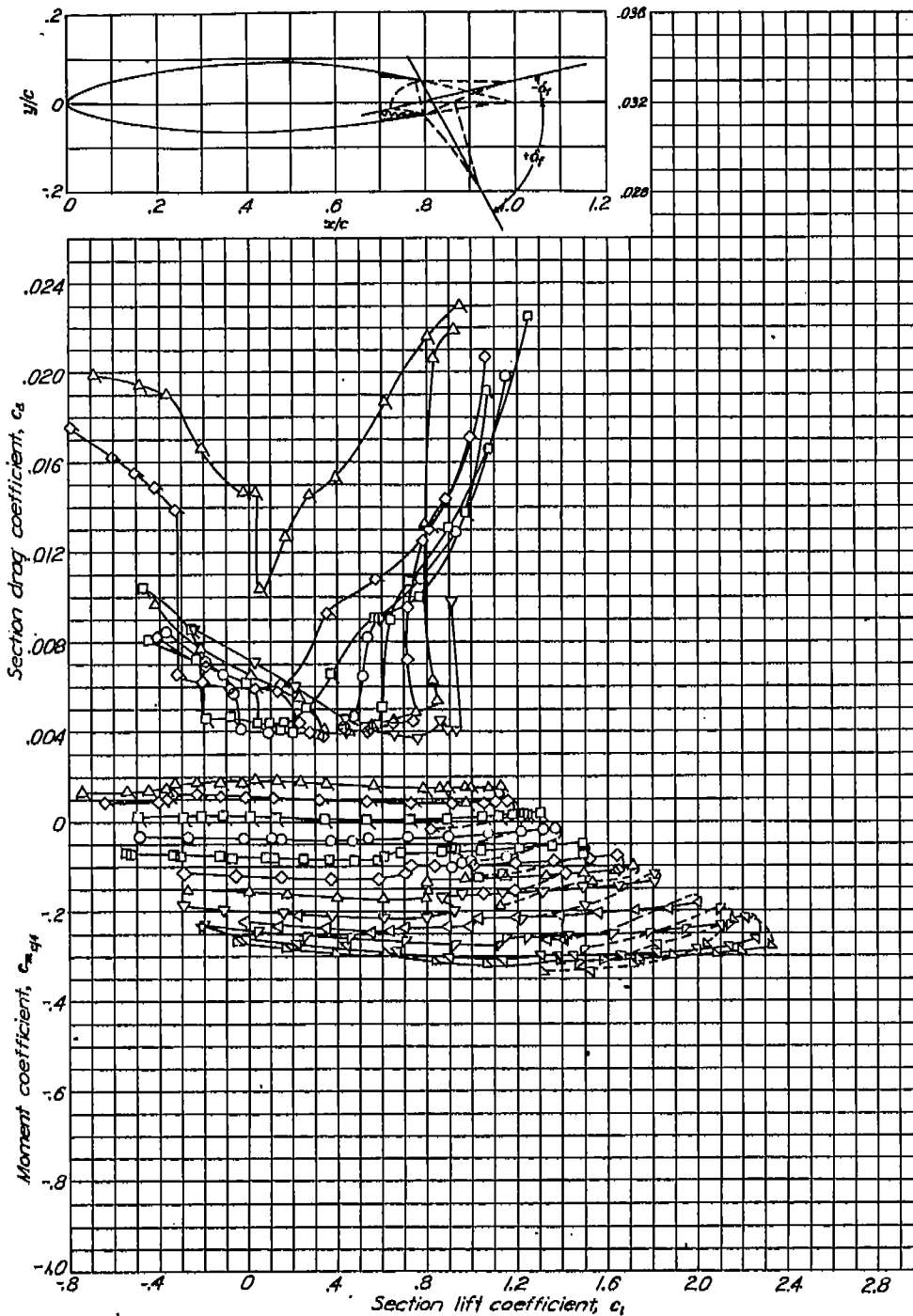
Aerodynamic characteristics of the NACA 66(215)-216 airfoil section with 0.20% sealed plain flap. R=6 \times 10^4 .
