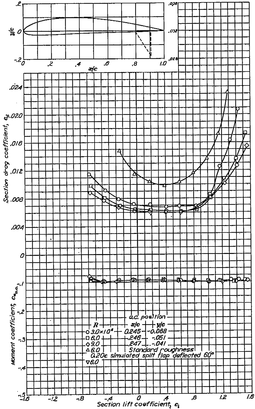
Aerodynamic characteristics of the NACA 4412 airfoil section, 24-inch chord.
