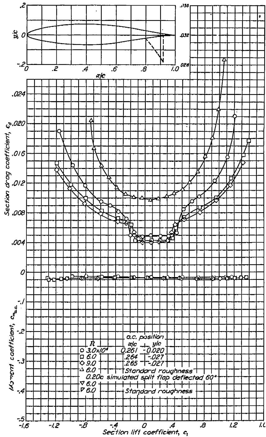
Aerodynamic characteristics of the NACA 65(215)-114 airfoil section, 24 inch chord.
