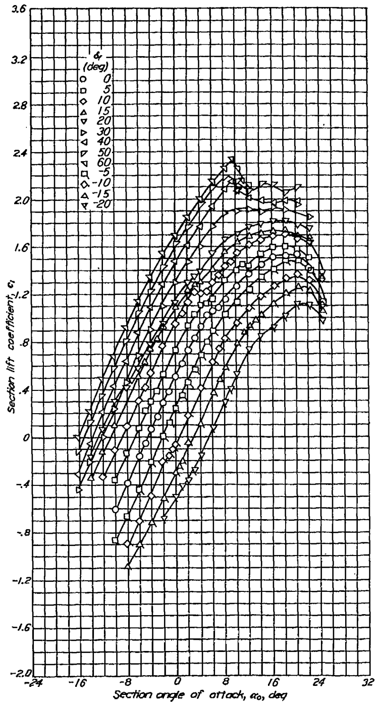
Aerodynamic characteristics of the NACA 65,3-618 airfoil section with 0.20c sealed plain flap. R=6 \times 10^6 .
