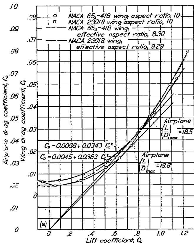
(a) NACA 65-418 and 23018 wings of aspect ratio 10.
