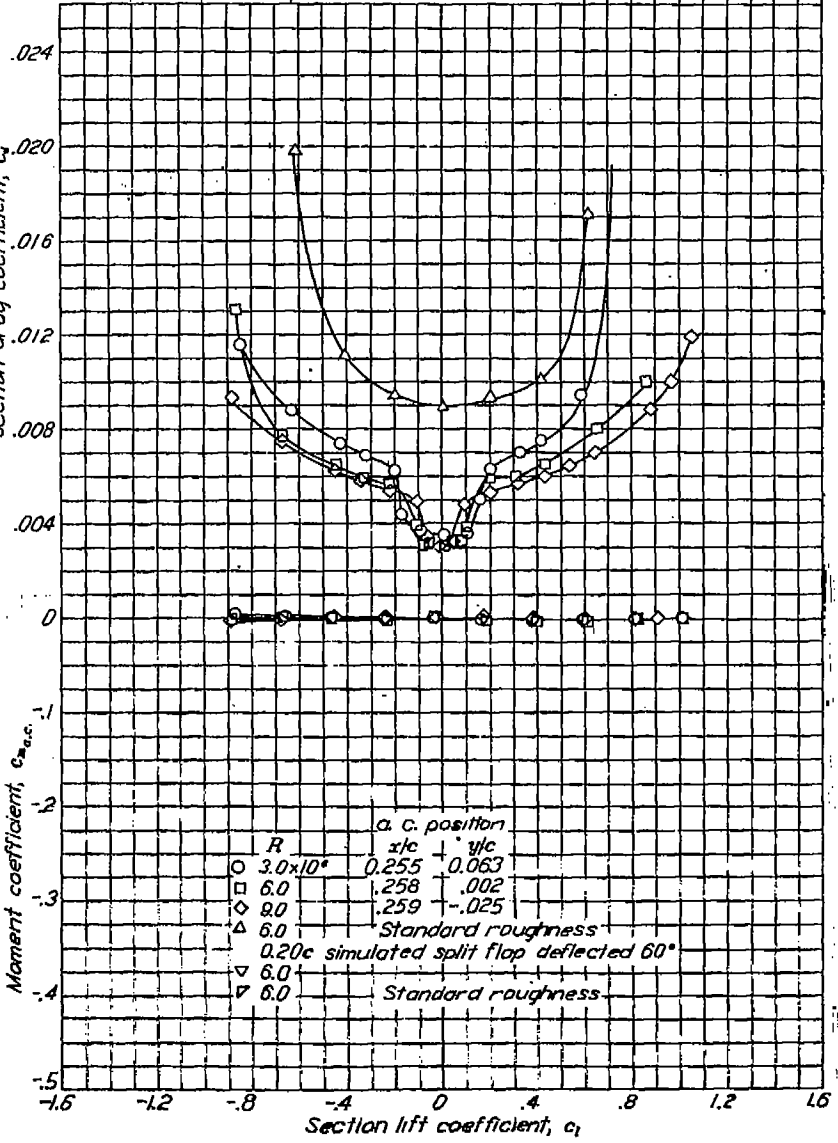
Aerodynamic characteristics of the NACA 66-009 airfoil section, 24-inch chord.
