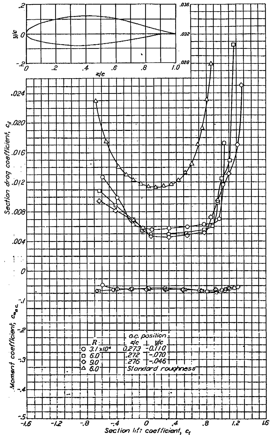
Aerodynamic characteristics of the NACA 65(421)-420 airfoil section, 24-inch chord.
