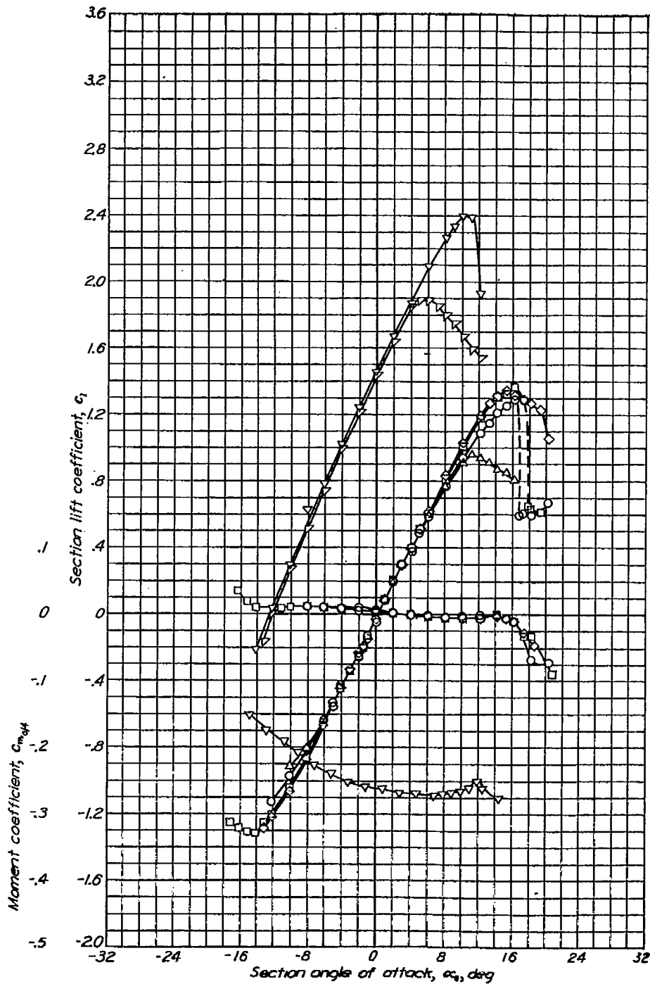
Aerodynamic characteristics of the NACA 66-015 airfoil section, 24-inch chord.
