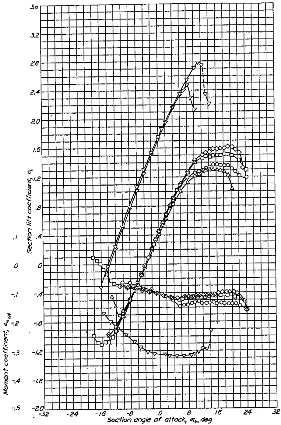
Aerodynamic characteristics of the NACA 64-618 airfoil section, 24-inch chord.
