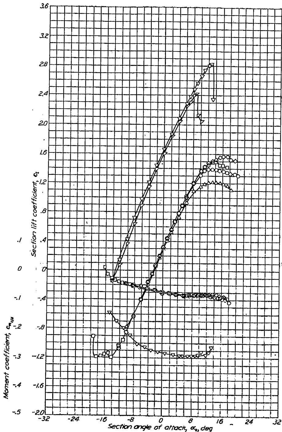
Aerodynamic characteristics of the NACA 63-418 airfoil section, 24-inch chord.
