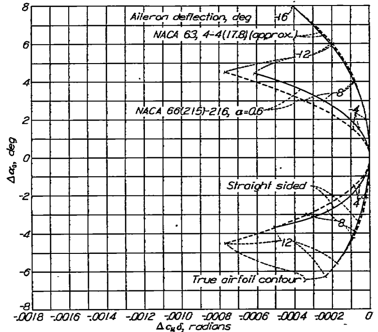
FIGURE 61.—Variation of the hinge-moment parameter \Delta c_H \delta with the equivalent change in section angle of attack required to maintain a constant section lift coefficient for deflection of true-airfoil-contour and straight-sided ailerons on the NACA 63,4-4(17.8) (approx.) and the NACA 66(215)-216, \alpha=0.6 airfoil sections. Gaps sealed.
