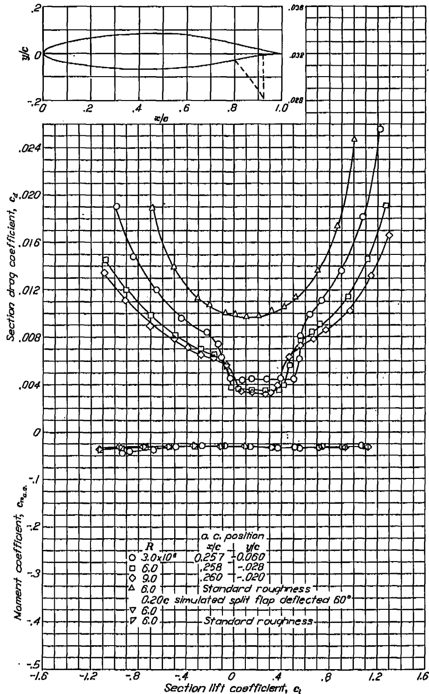
Aerodynamic characteristics of the NACA 662-215 airfoil section, 24-inch chord.
