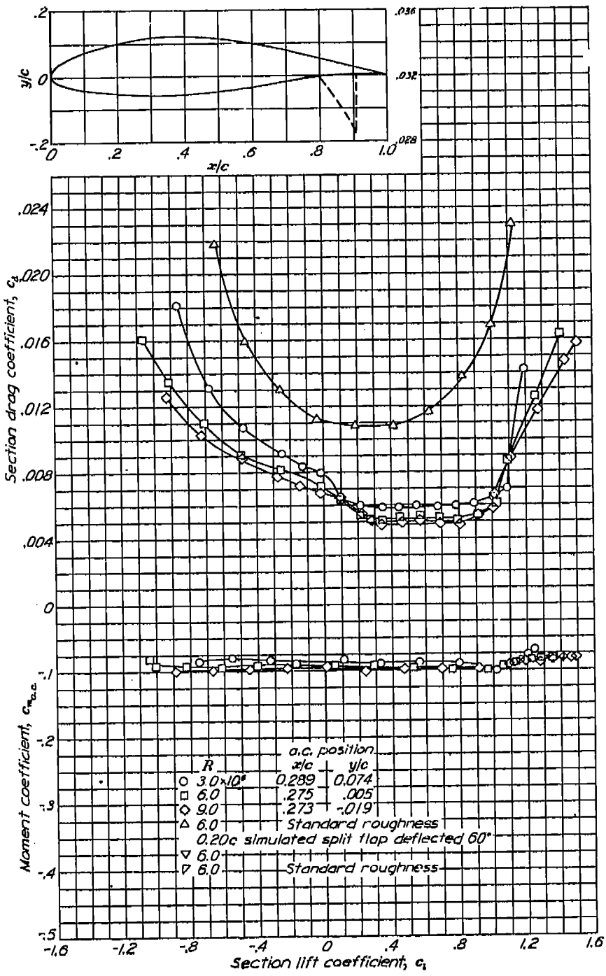
Aerodynamic characteristics of the NACA 64-618 airfoil section, 24-inch chord.
