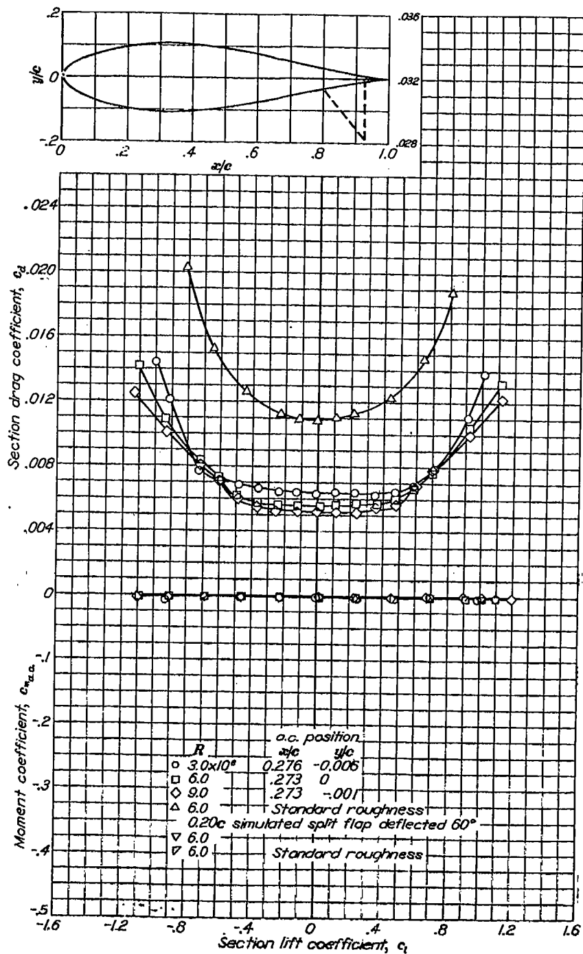
Aerodynamic characteristics of the NACA 63-021 airfoil section, 24-inch chord.
