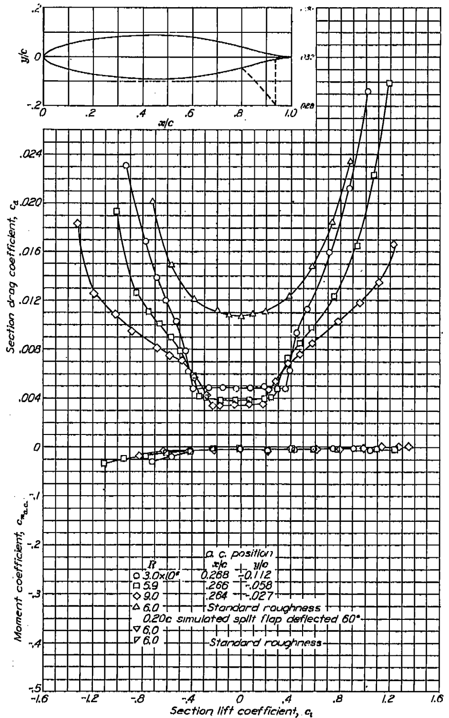
Aerodynamic characteristics of the NACA 663-018 airfoil section, 24-inch chord.
