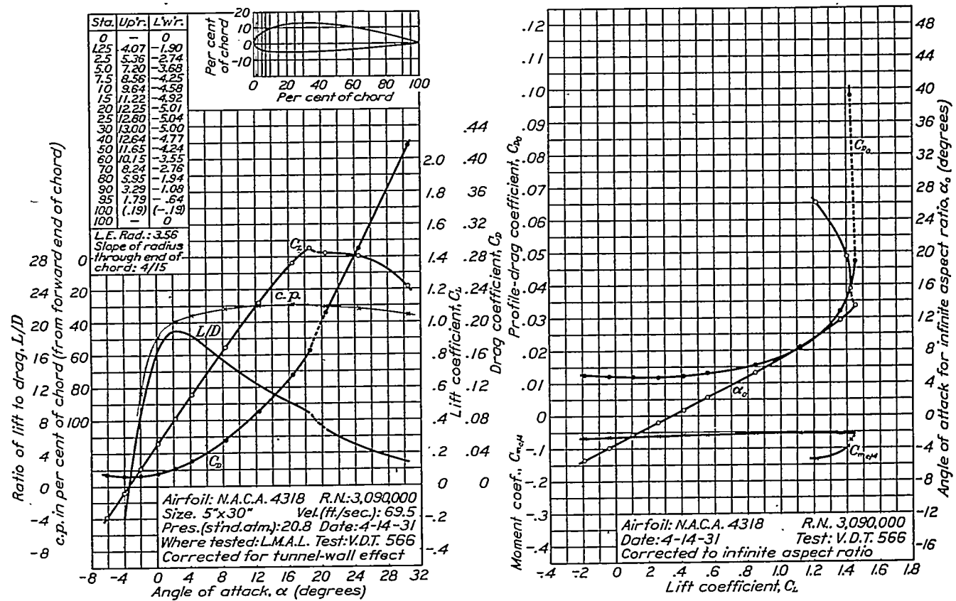
FIGURE 35.—N.A.C.A. 4318 airfoil.
