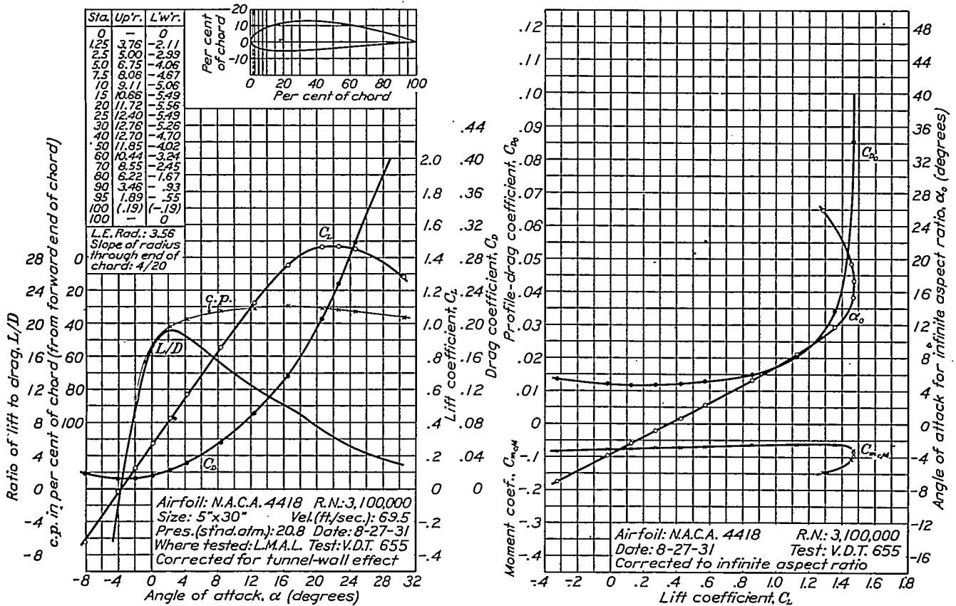
FIGURE 41.—N.A.C.A. 4418 airfoil.
