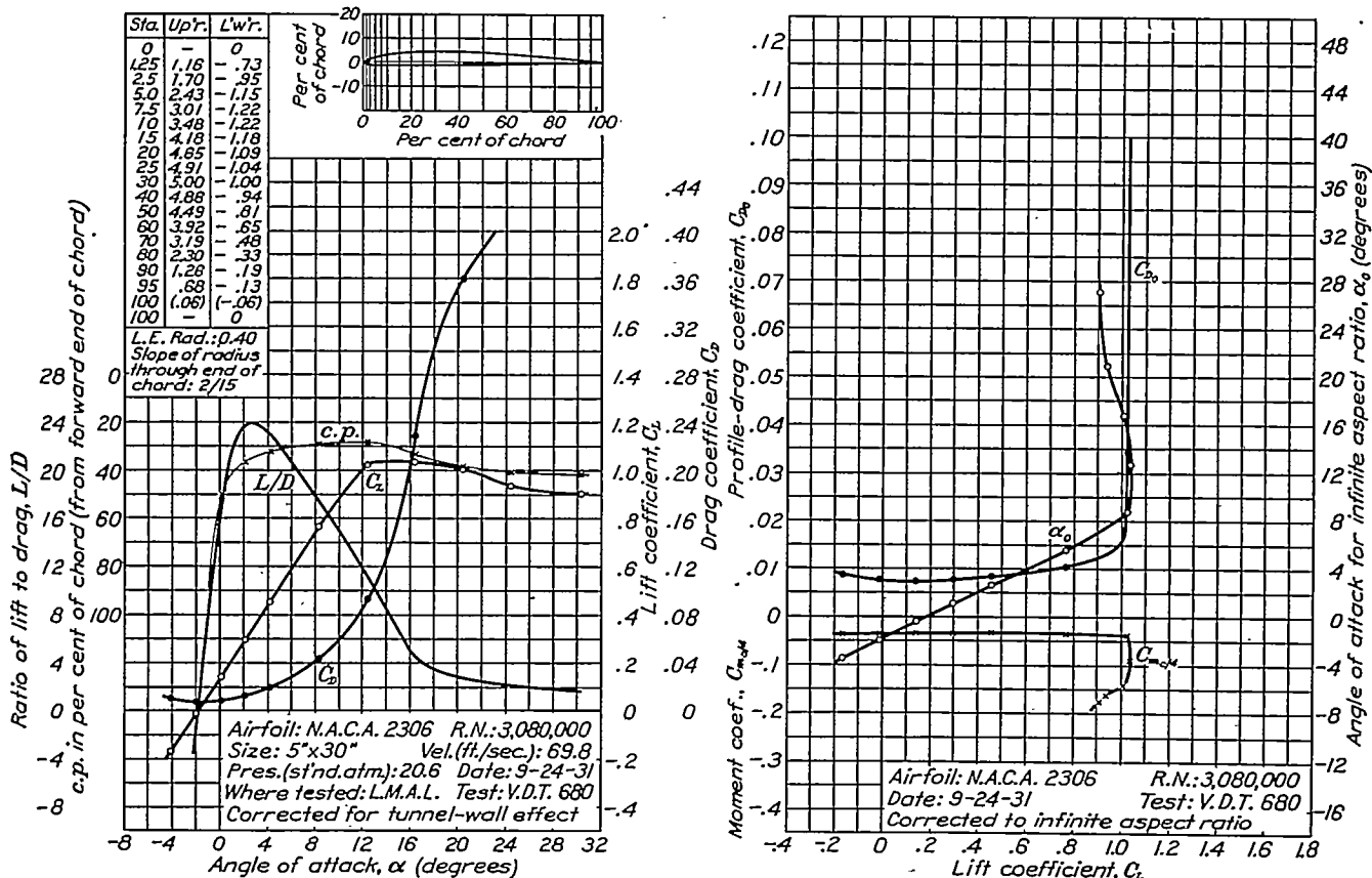
FIGURE 12.—N.A.C.A. 2306 airfoil.
