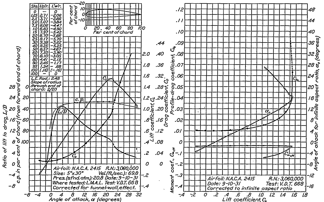
FIGURE 19.—N.A.C.A. 2415 airfoil.
