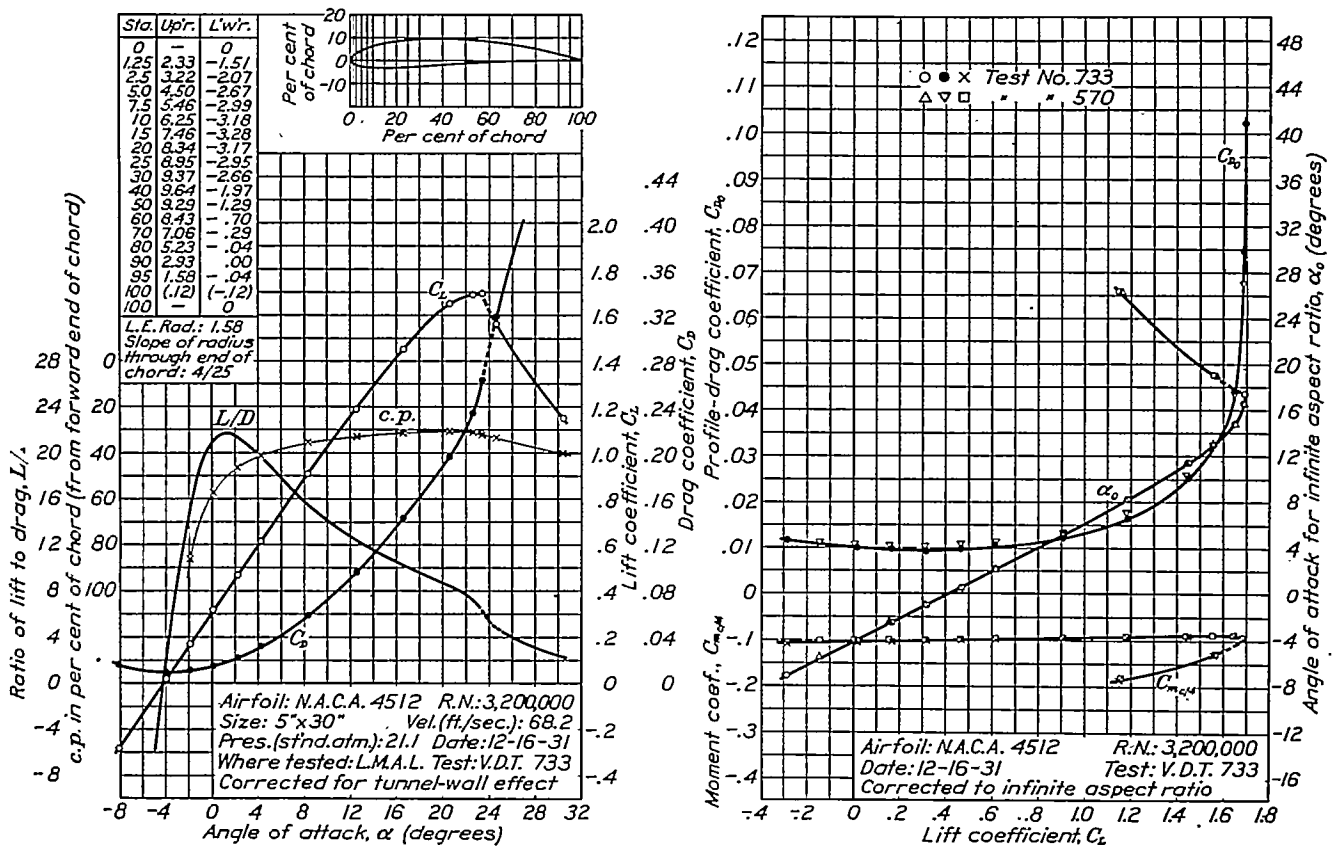
FIGURE 45.—N.A.C.A. 4512 airfoil.
