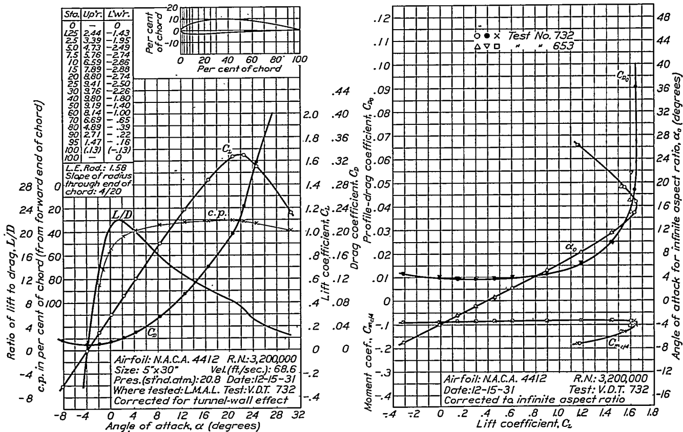
FIGURE 39.—N.A.C.A. 4412 airfoil.
