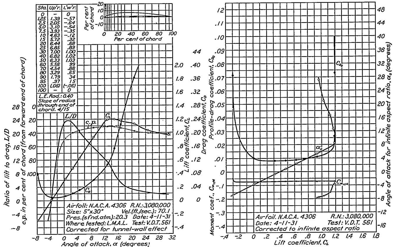
FIGURE 31.—N.A.C.A. 4306 airfoil.
