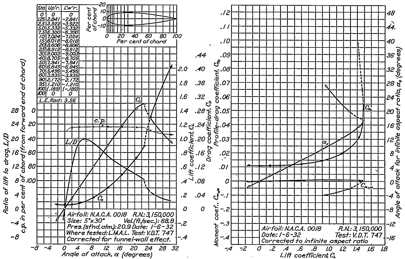
FIGURE 8.—N.A.C.A. 0018 airfoil.
