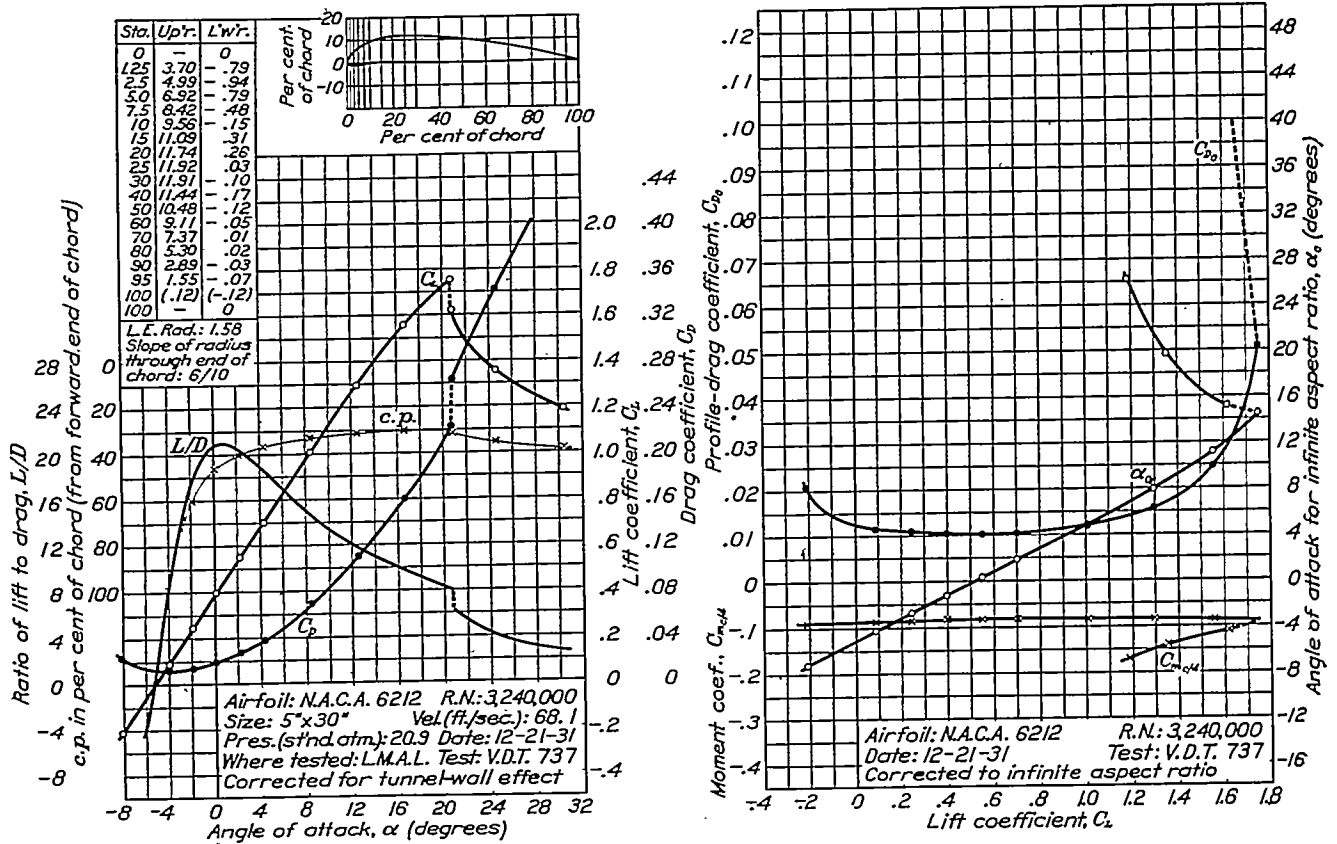
FIGURE 51.—N.A.C.A. 6212 airfoil.
