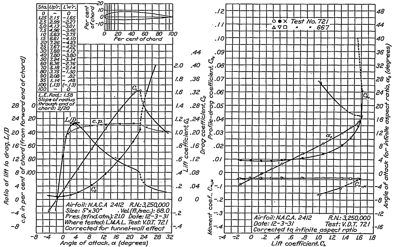
FIGURE 18.—N.A.C.A. 2412 airfoil.
