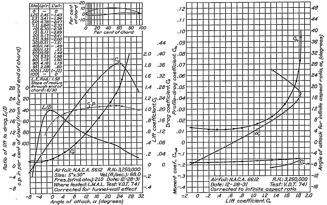
FIGURE 70.—N.A.C.A. 6612 airfoil.
