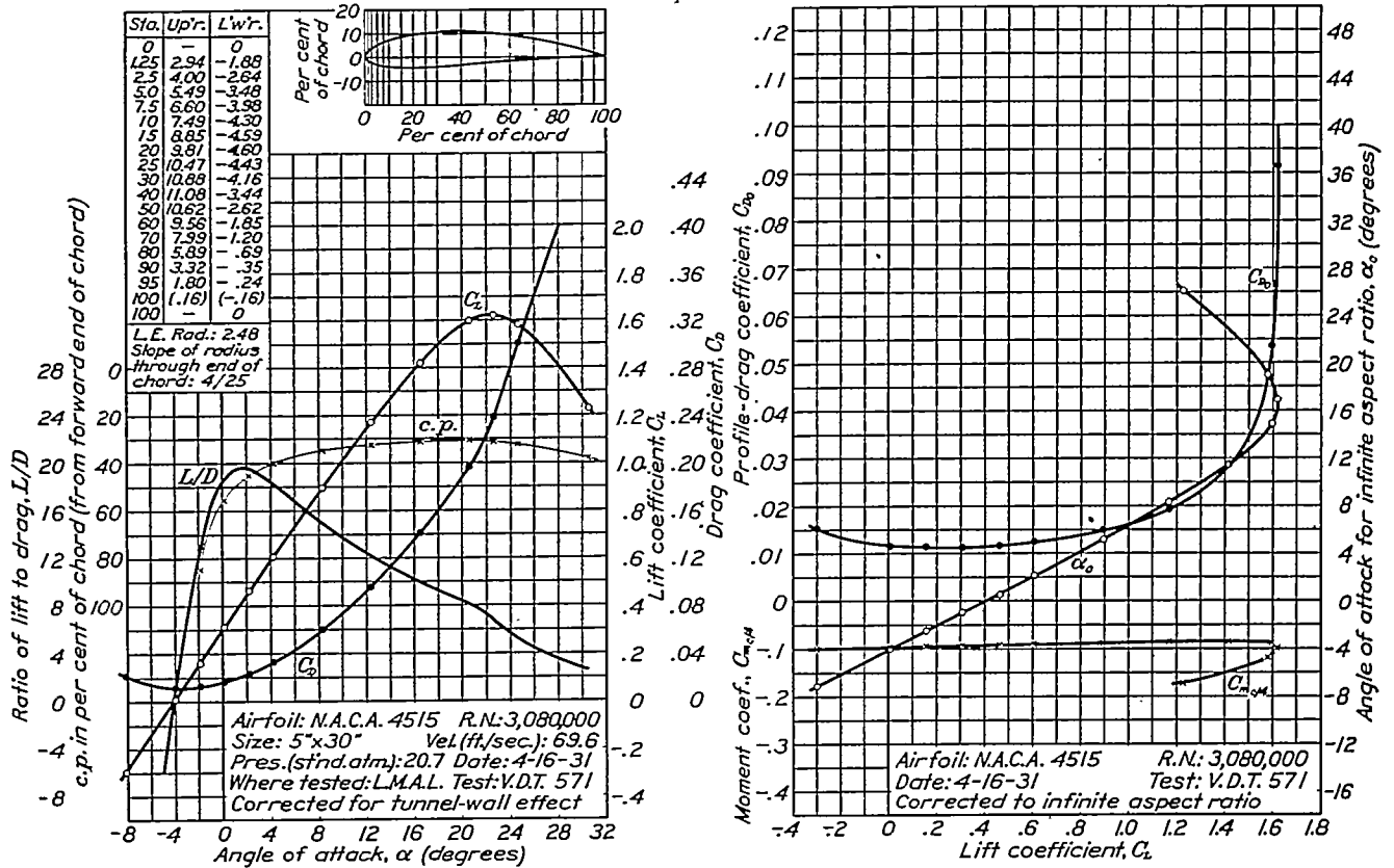
FIGURE 46.—N.A.C.A. 4515 airfoil.
