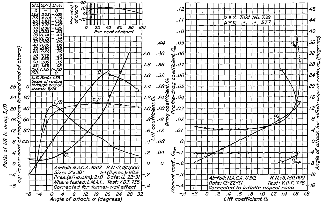
FIGURE 54.—N.A.C.A. 6312 airfoil.
