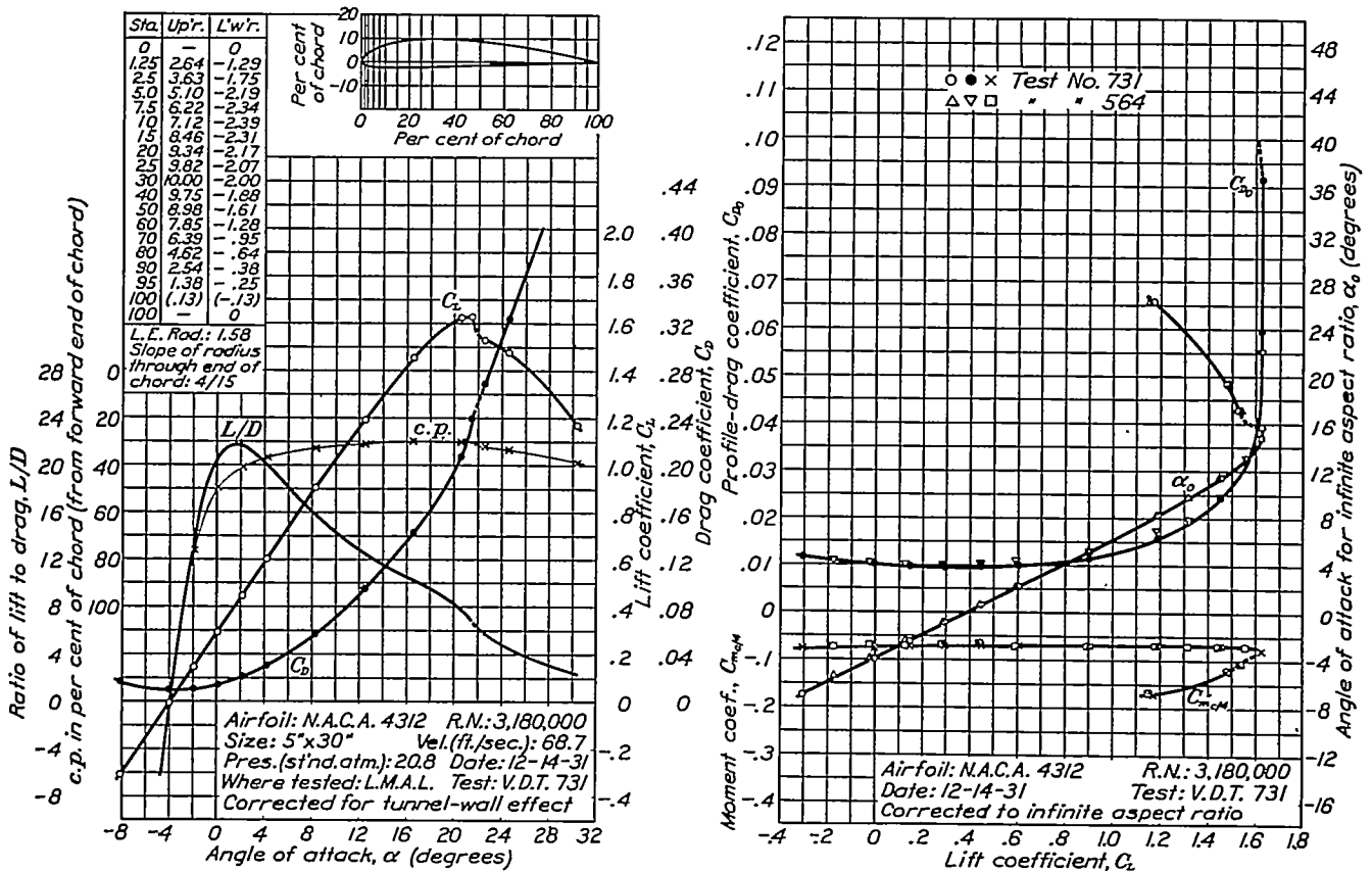
FIGURE 33.—N.A.C.A. 4312 airfoil.
