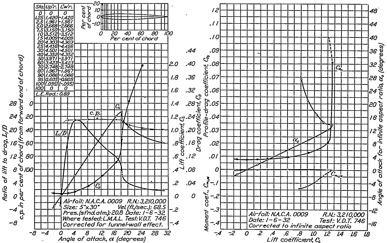
FIGURE 5.—N.A.C.A. 0009 airfoil.
