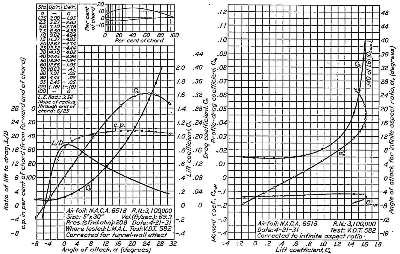
FIGURE 68.—N.A.C.A. 6518 airfoil.
