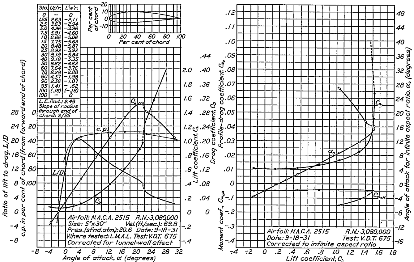
FIGURE 25.—N.A.C.A. 2515 airfoil.
