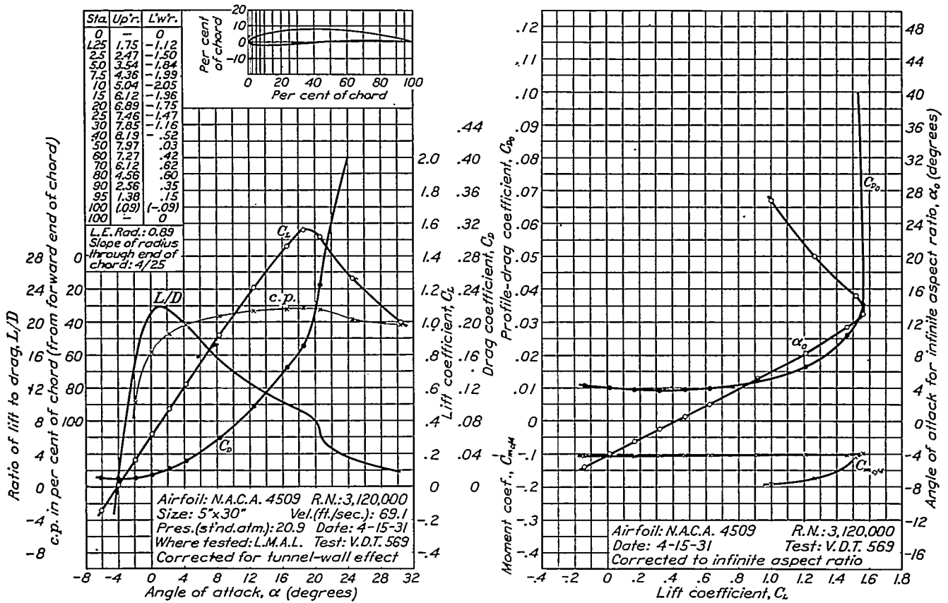
FIGURE 44.—N.A.C.A. 4509 airfoil.
