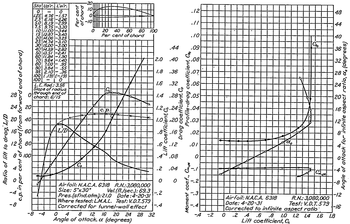
FIGURE 56.—N.A.O.A. 6318 airfoil.
