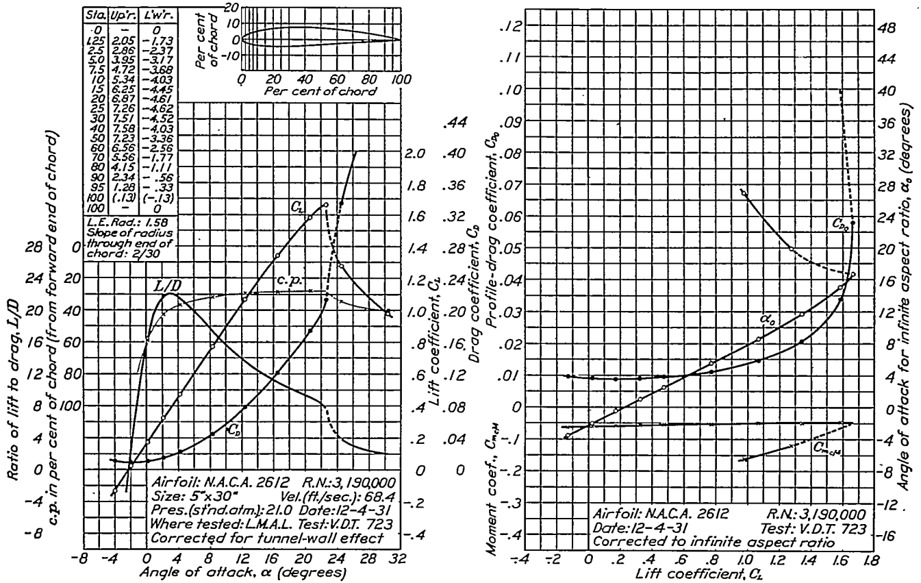
FIGURE 28.—N.A.C.A. 2612 airfoil.
