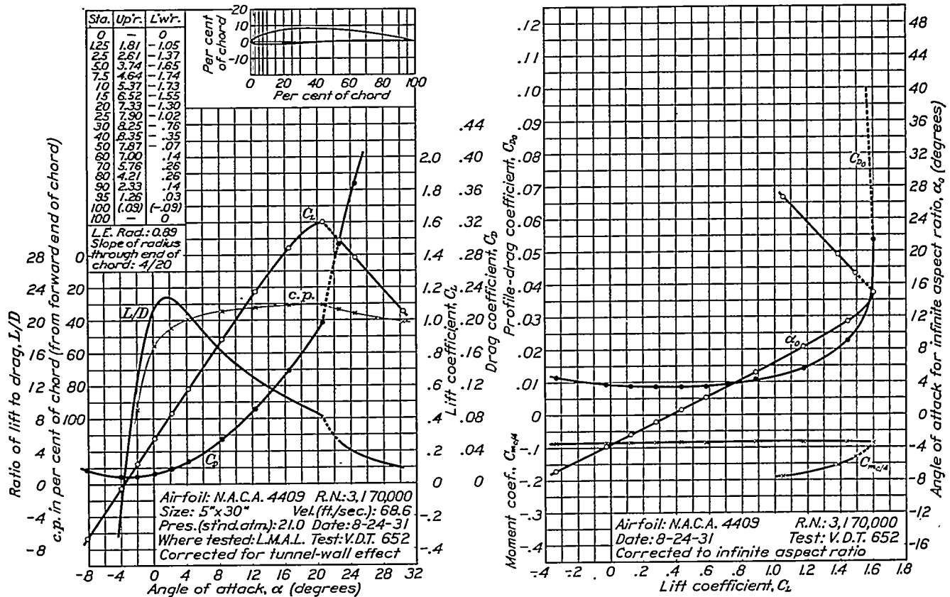
FIGURE 38.—N.A.C.A. 4409 airfoil.
