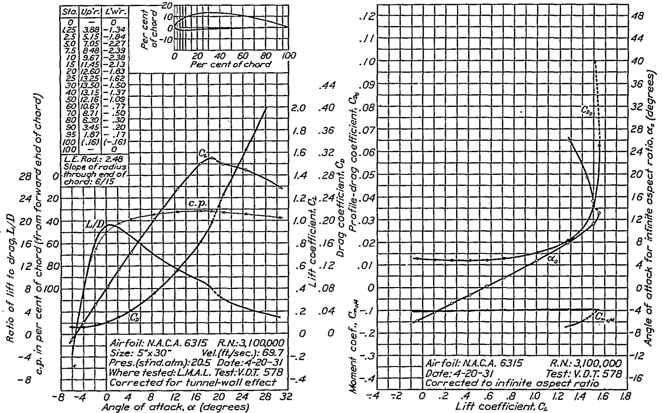
FIGURE 55.—N.A.C.A. 6315 airfoil.
