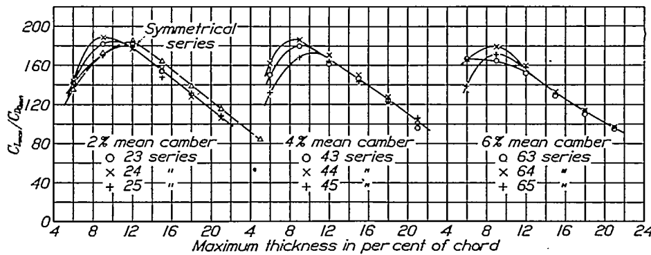
FIGURE 95.—Variation of C_{Lmax}/C_{D0min} with thickness.
