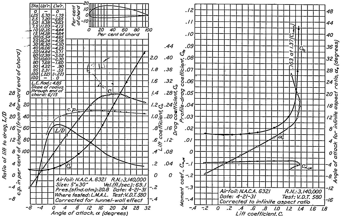
FIGURE 57.—N.A.O.A. 6321 airfoil.
