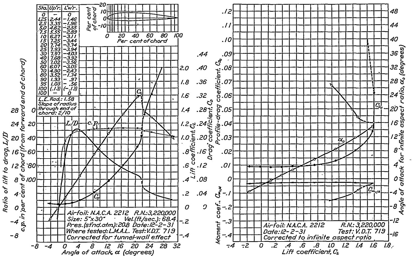
FIGURE 11.—N.A.O.A. 2212 airfoil.
