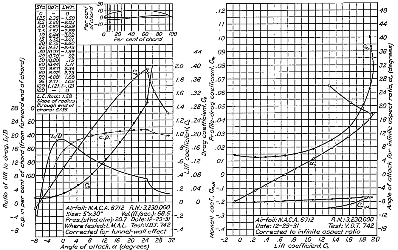
FIGURE 71.—N.A.C.A. 6712 airfoil.
