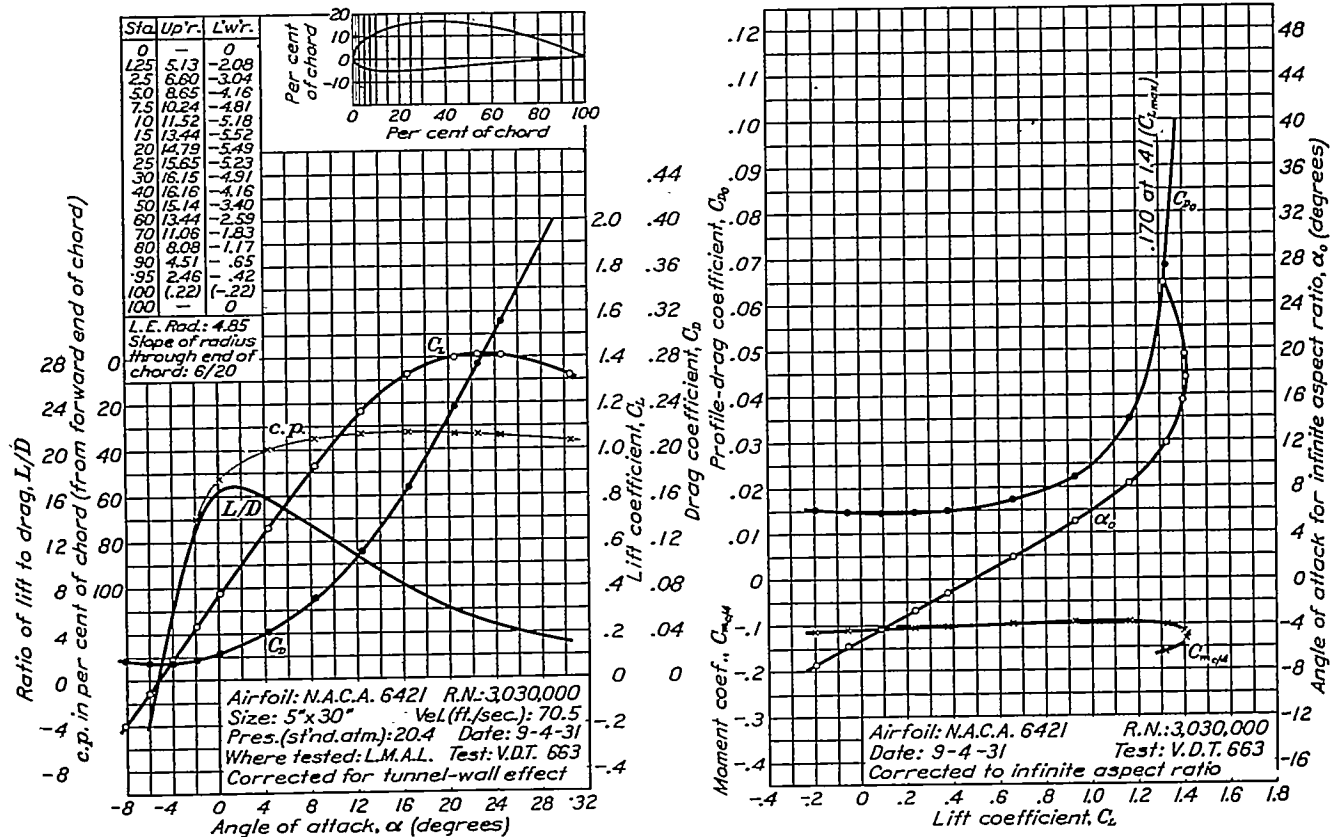
FIGURE 63.—N.A.C.A. 6421 airfoil.
