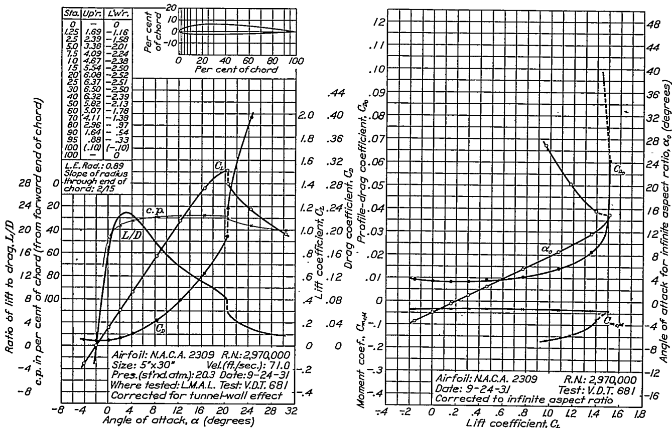
FIGURE 13.—N.A.C.A. 2309 airfoil.
