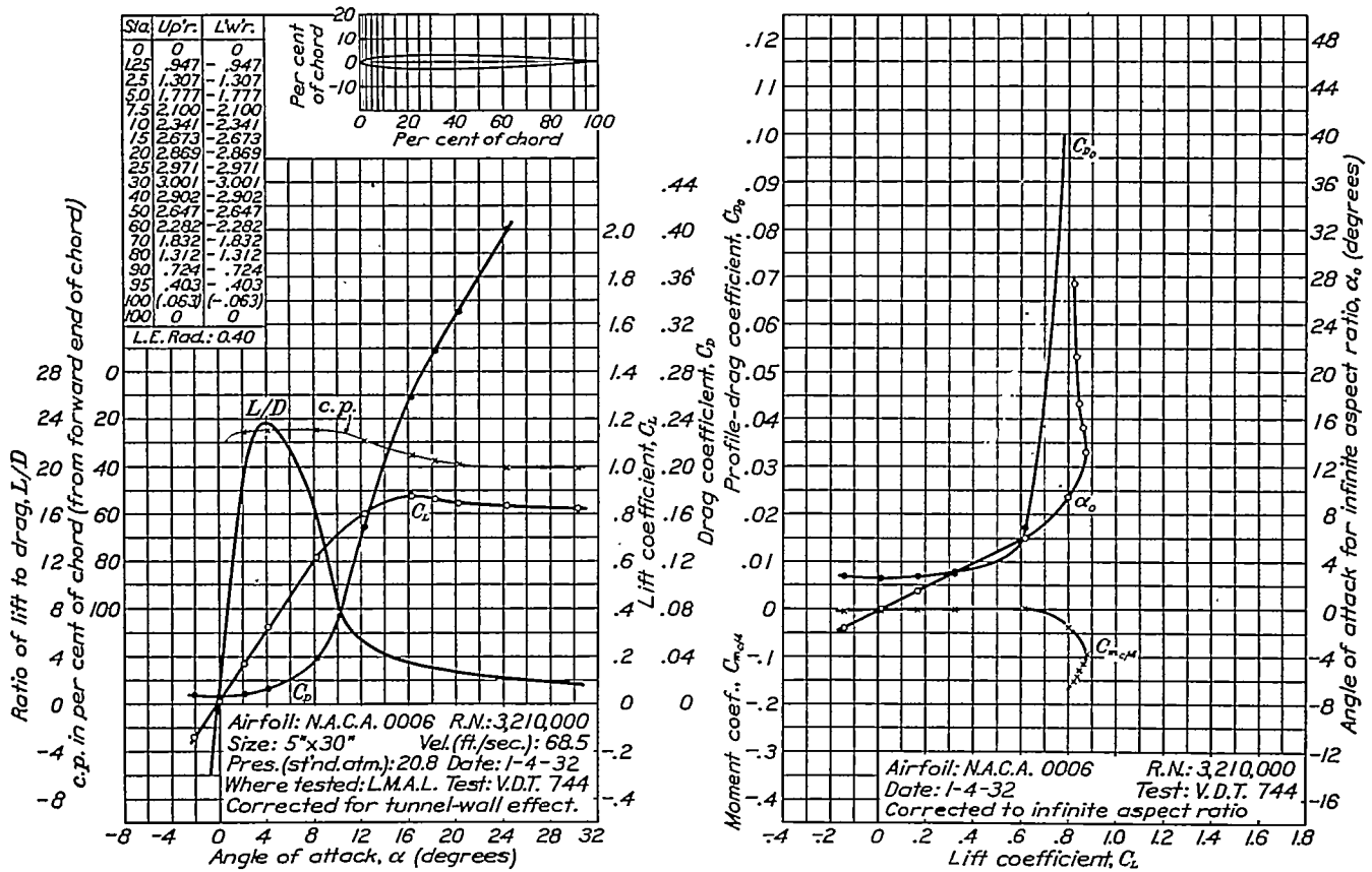
FIGURE 4.—N.A.C.A. 0006 airfoil.
