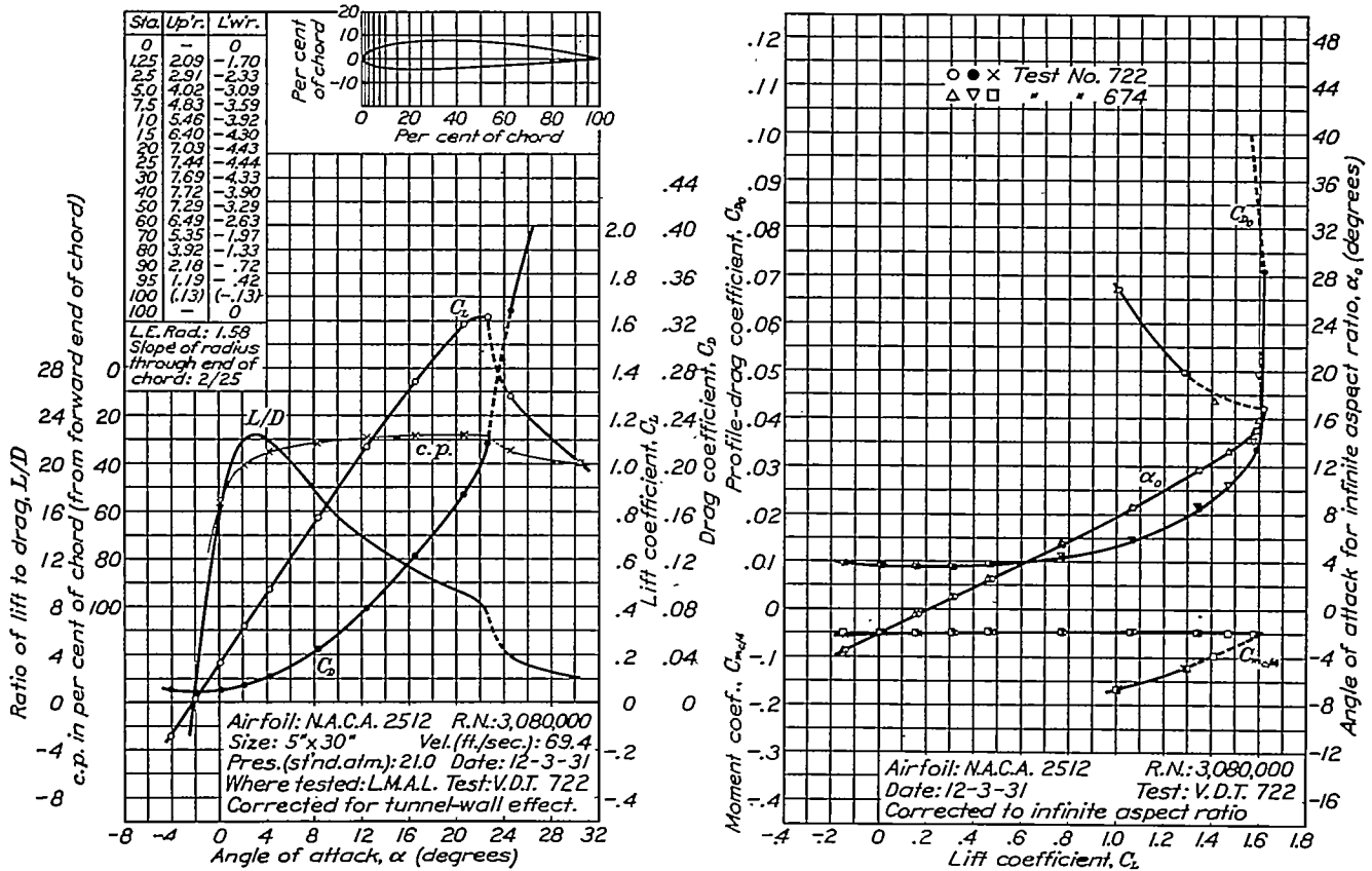
FIGURE 24.—N.A.C.A. 2512 airfoil.
