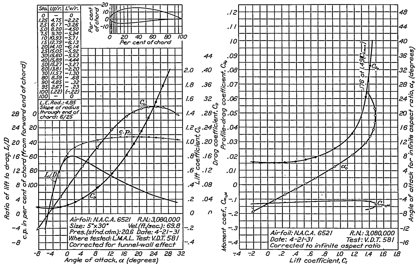
FIGURE 69.—N.A.C.A. 6521 airfoil.
