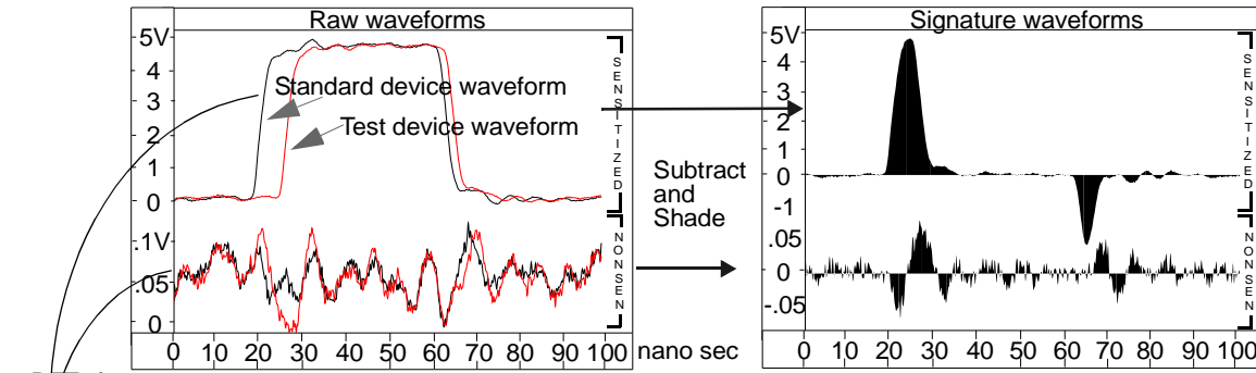
Figure 1. Time Domain Signature Waveform creation procedure.
