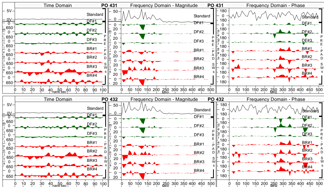
Figure 6. Time and Frequency domain Signature Waveforms from PO 431 and 432 of Bridging Exp. #1.
