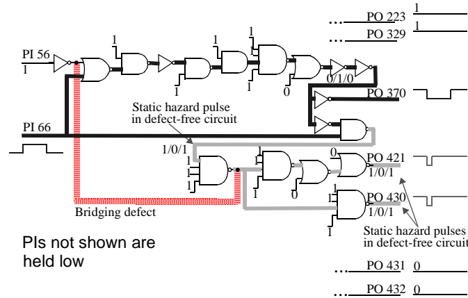
Figure 4. Portions of the c432 schematic showing the short and the sensitized paths affected by the defect of Bridging Experiment #1.
