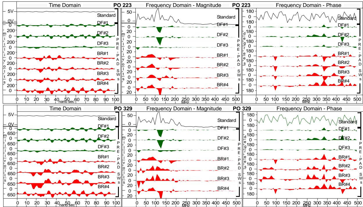
Figure 5. Time and Frequency domain Signature Waveforms from POs 223 and 329 of Bridging Exp. #1.
