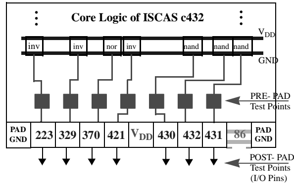
Figure 3. Location of the test points on the c432.
