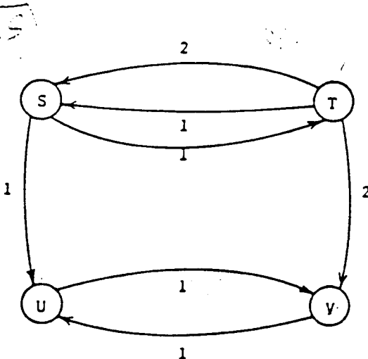
FIG. 1. Example of a system in which process P_2 can deadlock. The set of states is \Sigma = \{S, T, U, V\} , and the set of processes is \Pi = \{P_1, P_2\} .
