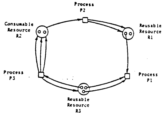
FIG. 4. Example of a state in a general resource system. R_1 and R_3 are reusable resources whose total units are t_1 = 2 and t_3 = 3 . R_2 is a consumable resource whose only producer is P_2 . The available units are r_1 = 1 , r_2 = 2 , and r_3 = 0 . The state is not deadlocked because it can be reduced by P_1 , then by P_2 , and then by P_3 .
