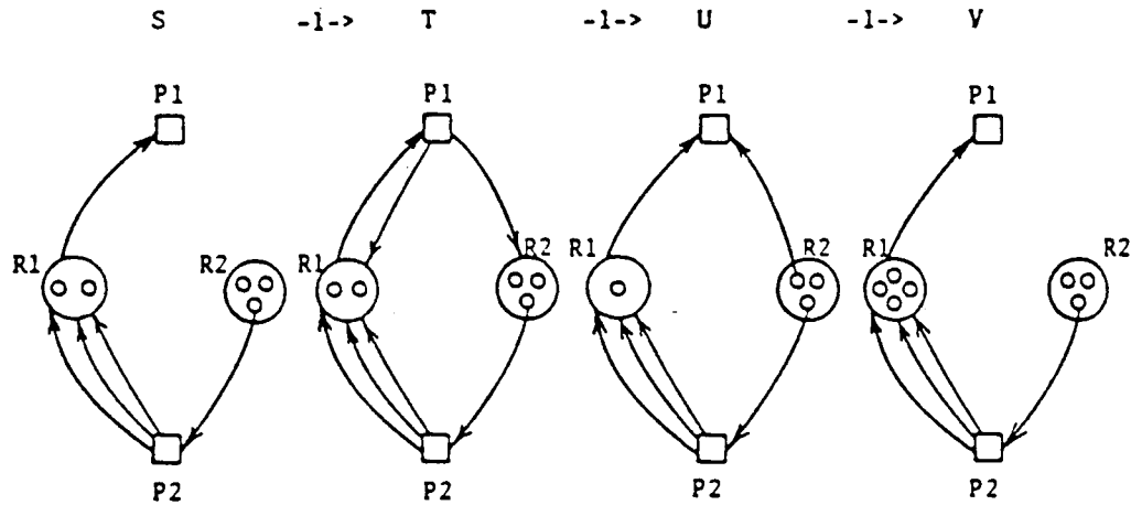
FIG. 5. Examples of operations in a general resource system. The system consists of consumable resource R1 (whose only producer is process P1), reusable resource R2 (which has three total units), and processes P1 and P2. Process P1 changes the state first by requesting one unit of each resource, next by acquiring the two units, and finally by releasing three units of R1 plus the acquired unit of R2. Process P2 is blocked in S because it has requested more units than are available , but P2 is no longer blocked in state V .
