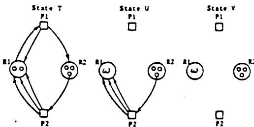
FIG. 6. Reductions of a general resource graph. (State T is identical to state T in Figure 5.) R_1 is a consumable resource, and R_2 is a reusable resource. State T is reduced by P_1 to obtain U , and U is reduced by P_2 to obtain V . T is completely reducible because the reductions delete all edges; therefore, T is not a deadlock state.
