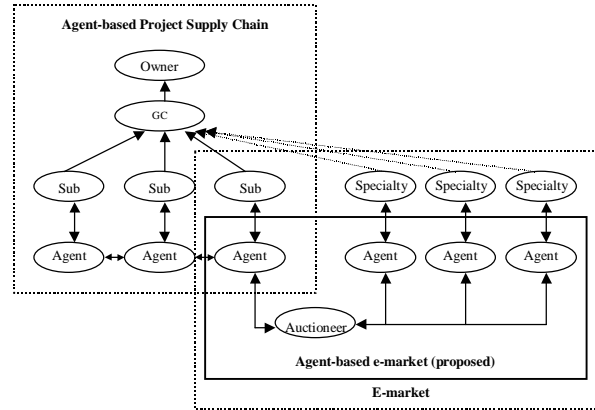
Figure 2. Agent-based e-Market Framework
